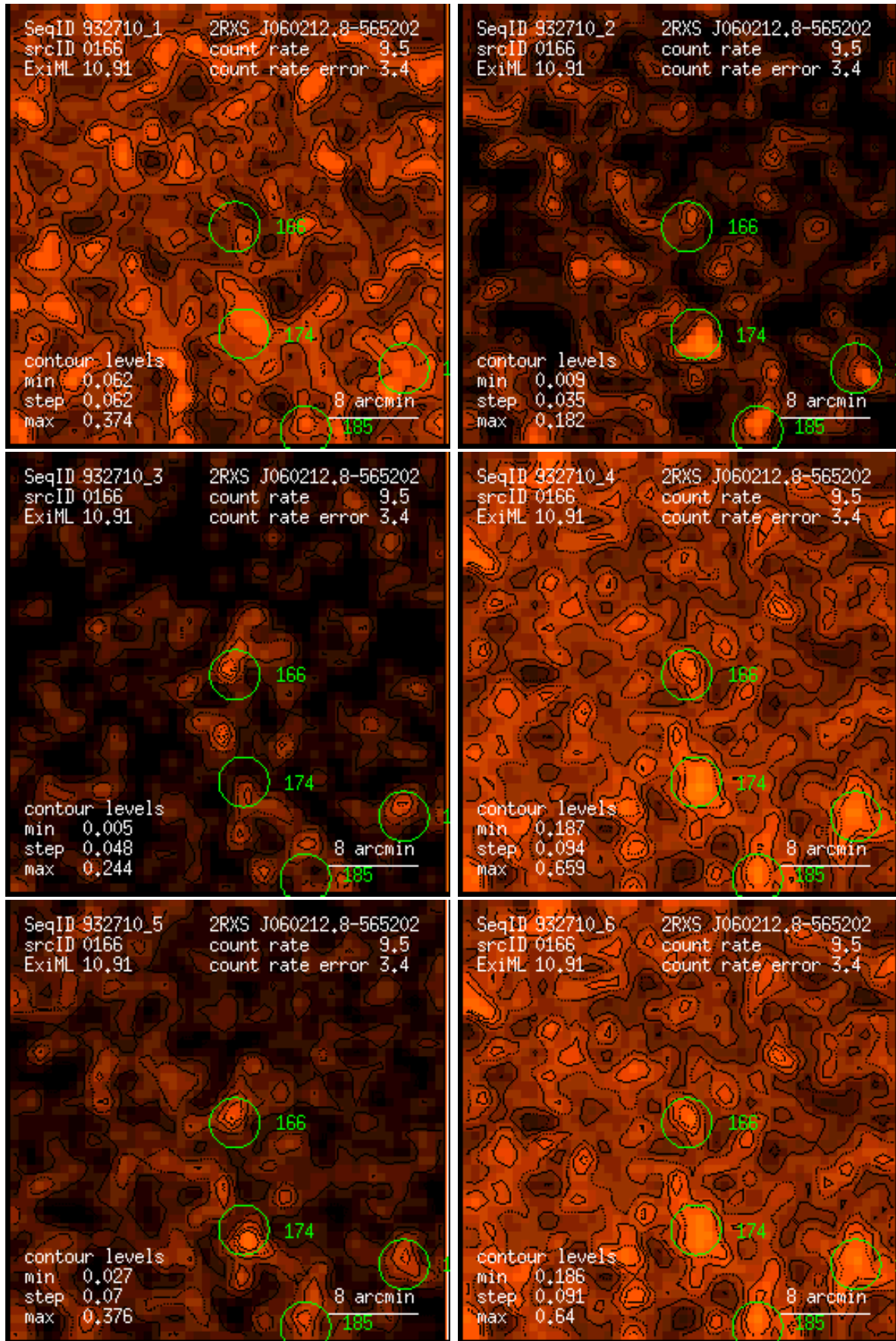
Figure 166: RASS 932710: detection 0166: band rate images, Gaussian filter: (1) PSPC channels 11 – 41, (2) 52 – 90, (3) 91 – 201, (4) 11 – 235, (5) 52 – 201, (6) 11 – 201. Broad band rates in counts/ks. Band rate contour levels in counts/ks/arcmin 2 .
