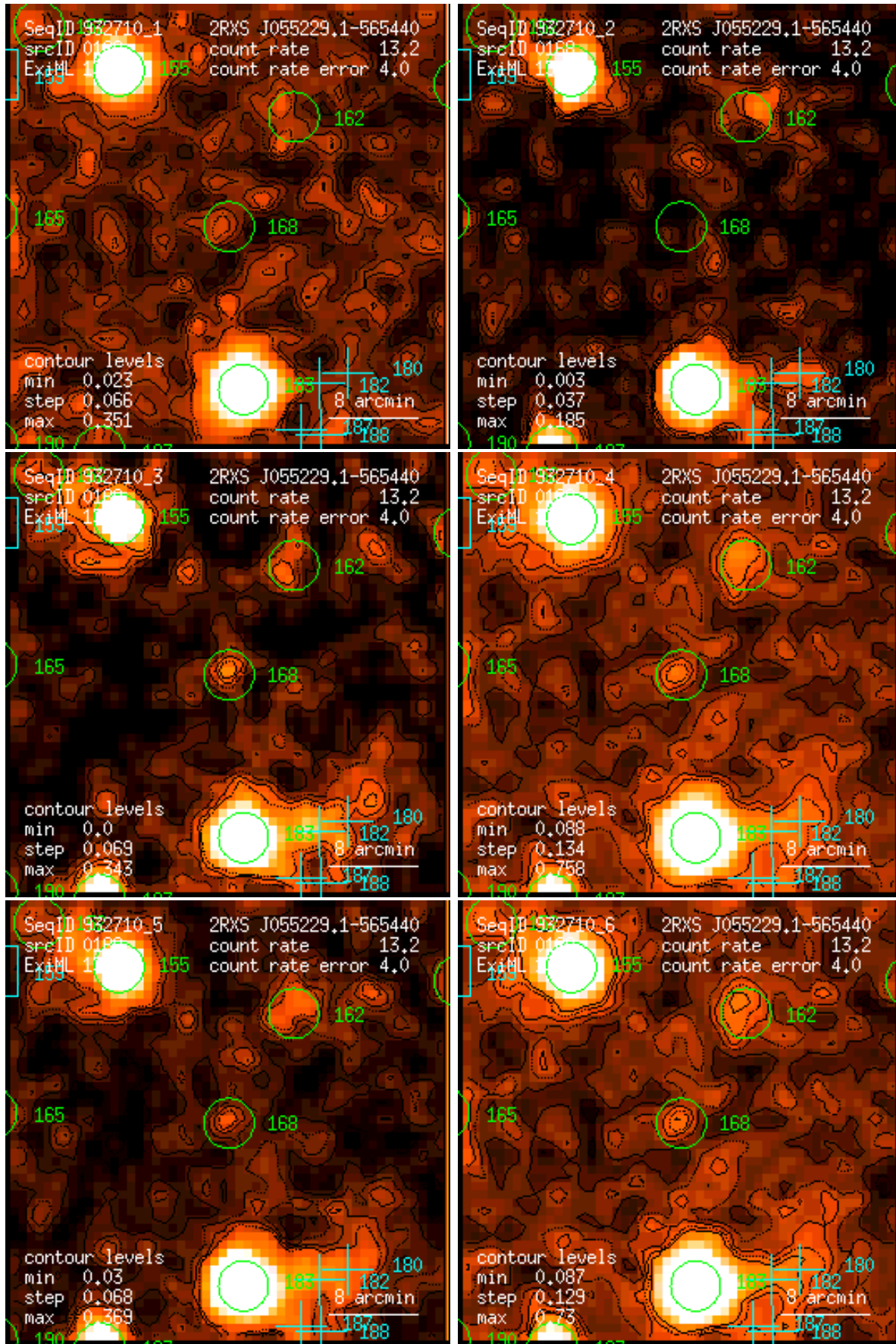
Figure 168: RASS 932710: detection 0168: band rate images, Gaussian filter: (1) PSPC channels 11 – 41, (2) 52 – 90, (3) 91 – 201, (4) 11 – 235, (5) 52 – 201, (6) 11 – 201. Broad band rates in counts/ks. Band rate contour levels in counts/ks/arcmin 2 .
