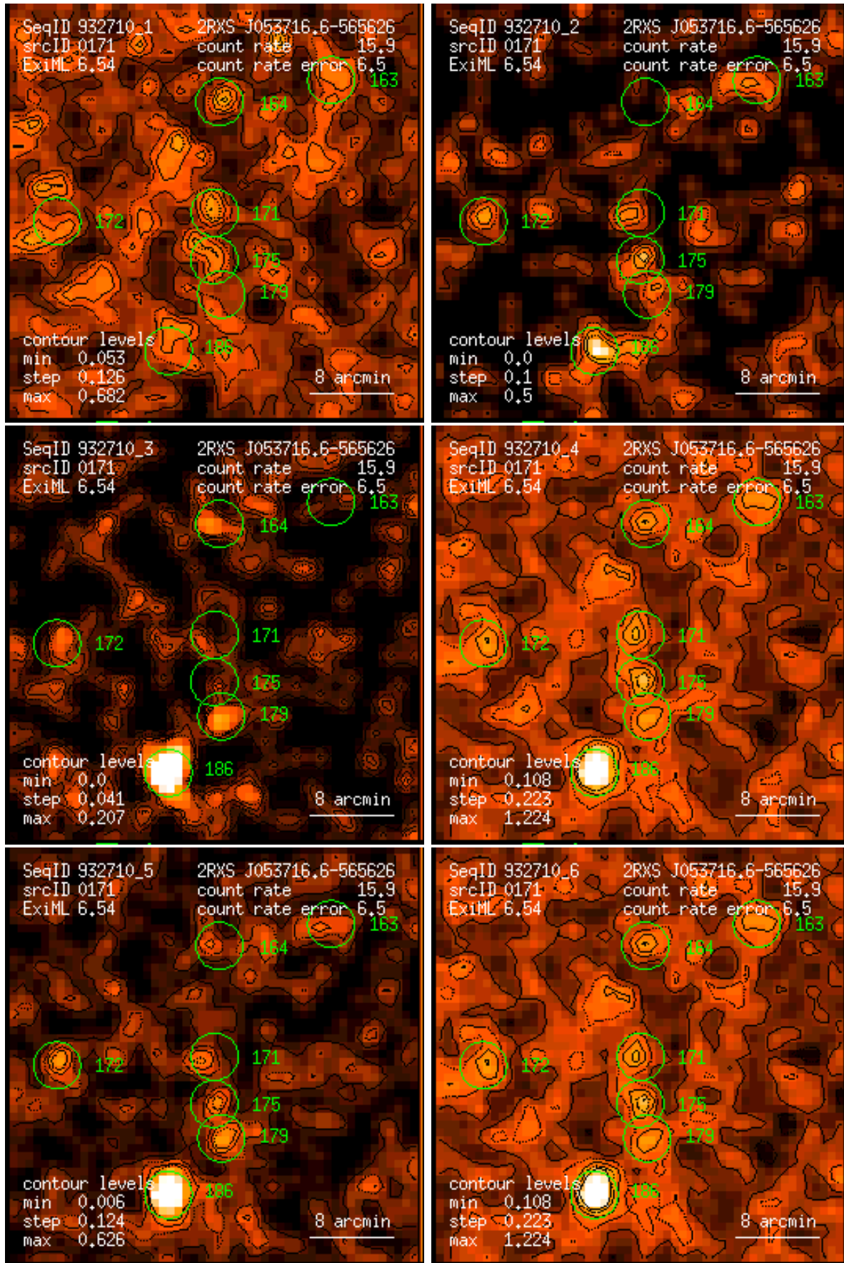
Figure 171: RASS 932710: detection 0171: band rate images, Gaussian filter: (1) PSPC channels 11 – 41, (2) 52 – 90, (3) 91 – 201, (4) 11 – 235, (5) 52 – 201, (6) 11 – 201. Broad band rates in counts/ks. Band rate contour levels in counts/ks/arcmin 2 .
