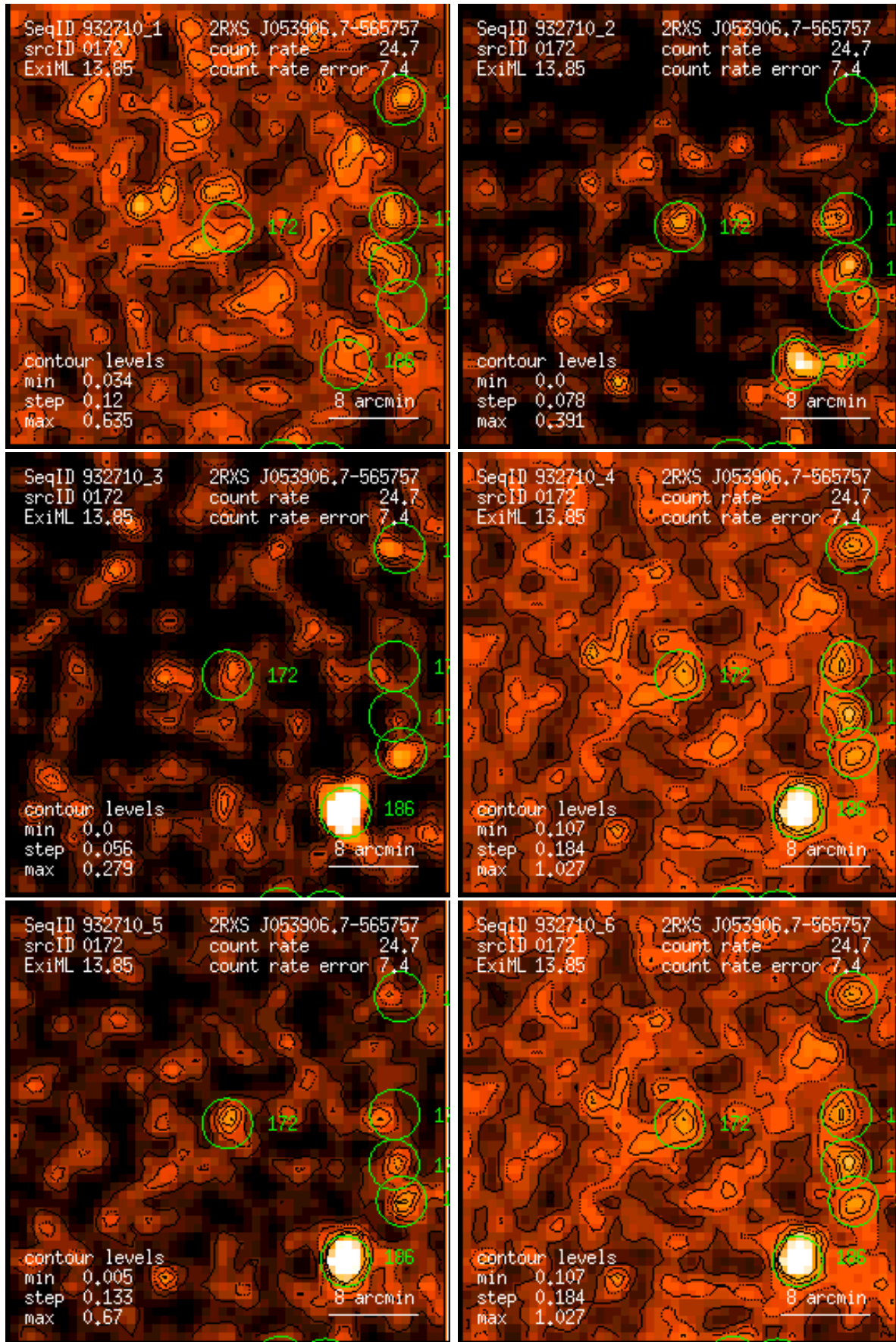
Figure 172: RASS 932710: detection 0172: band rate images, Gaussian filter: (1) PSPC channels 11 – 41, (2) 52 – 90, (3) 91 – 201, (4) 11 – 235, (5) 52 – 201, (6) 11 – 201. Broad band rates in counts/ks. Band rate contour levels in counts/ks/arcmin 2 .
