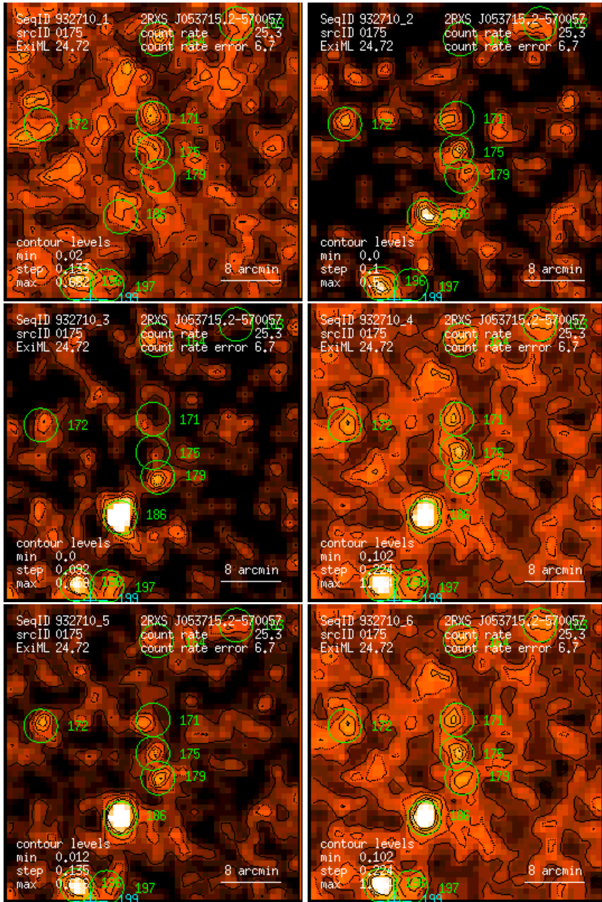
Figure 175: RASS 932710: detection 0175: band rate images, Gaussian filter: (1) PSPC channels 11 – 41, (2) 52 – 90, (3) 91 – 201, (4) 11 – 235, (5) 52 – 201, (6) 11 – 201. Broad band rates in counts/ks. Band rate contour levels in counts/ks/arcmin 2 .
