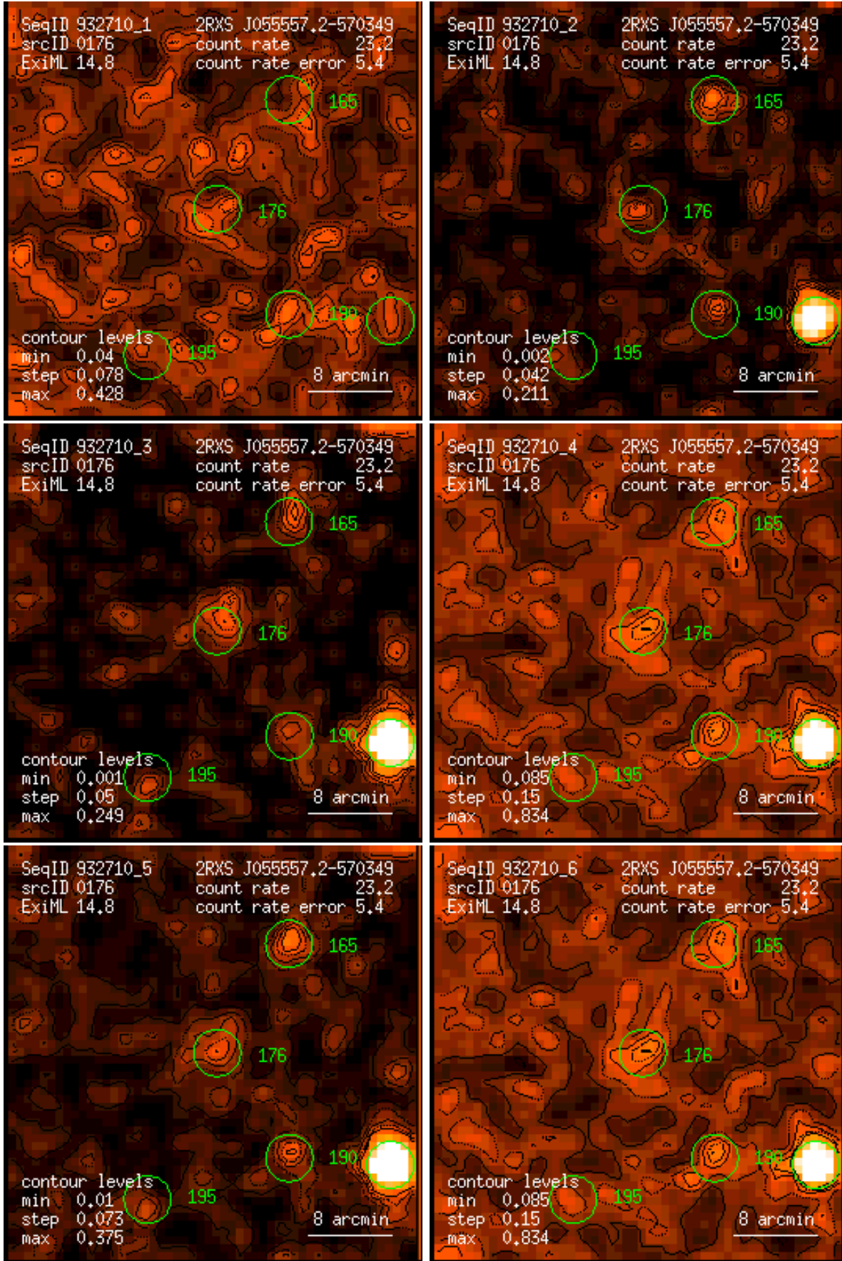
Figure 176: RASS 932710: detection 0176: band rate images, Gaussian filter: (1) PSPC channels 11 – 41, (2) 52 – 90, (3) 91 – 201, (4) 11 – 235, (5) 52 – 201, (6) 11 – 201. Broad band rates in counts/ks. Band rate contour levels in counts/ks/arcmin 2 .
