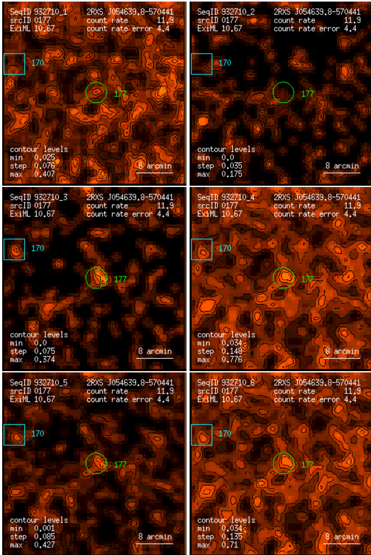
Figure 177: RASS 932710: detection 0177: band rate images, Gaussian filter: (1) PSPC channels 11 – 41, (2) 52 – 90, (3) 91 – 201, (4) 11 – 235, (5) 52 – 201, (6) 11 – 201. Broad band rates in counts/ks. Band rate contour levels in counts/ks/arcmin 2 .
