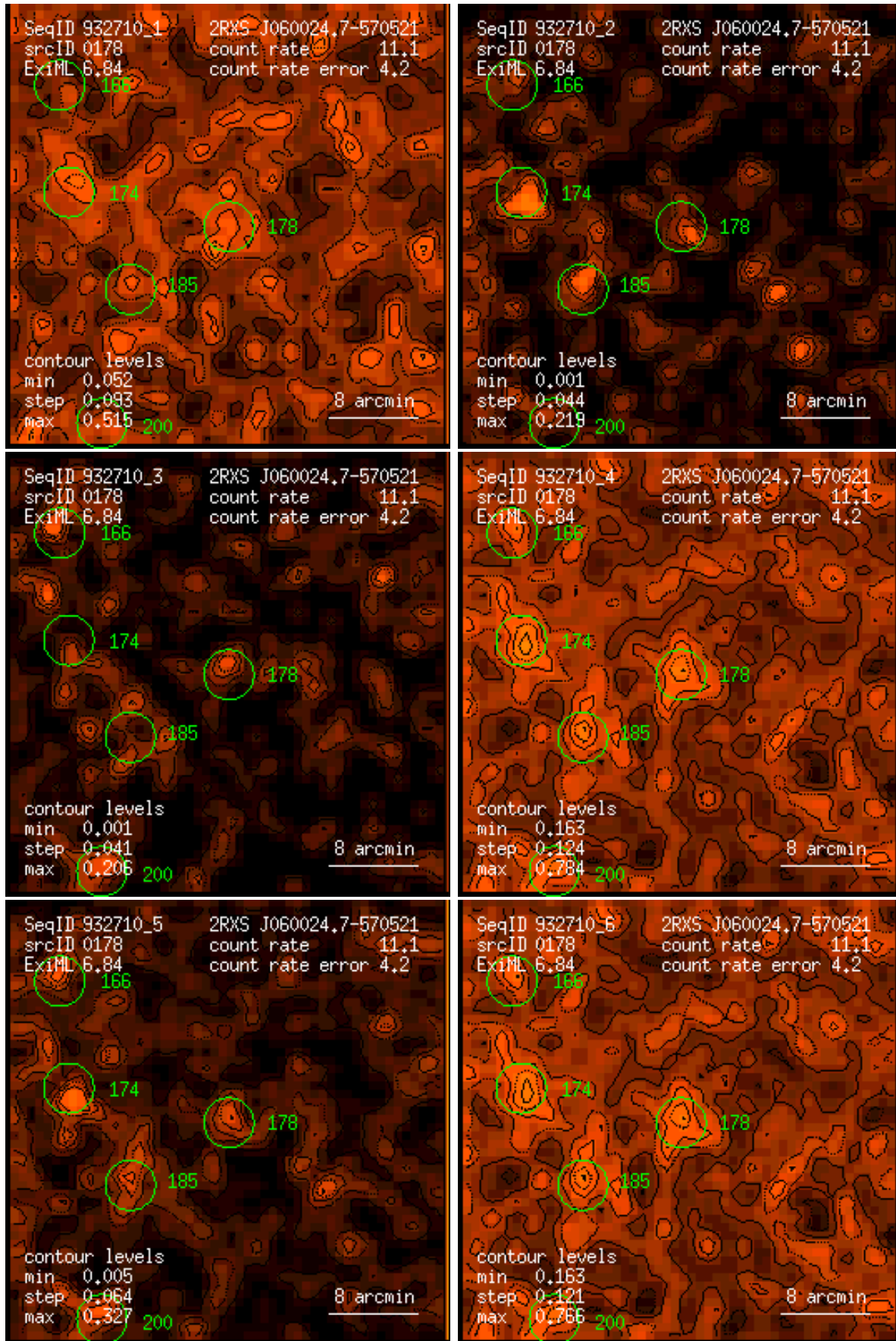
Figure 178: RASS 932710: detection 0178: band rate images, Gaussian filter: (1) PSPC channels 11 – 41, (2) 52 – 90, (3) 91 – 201, (4) 11 – 235, (5) 52 – 201, (6) 11 – 201. Broad band rates in counts/ks. Band rate contour levels in counts/ks/arcmin 2 .
