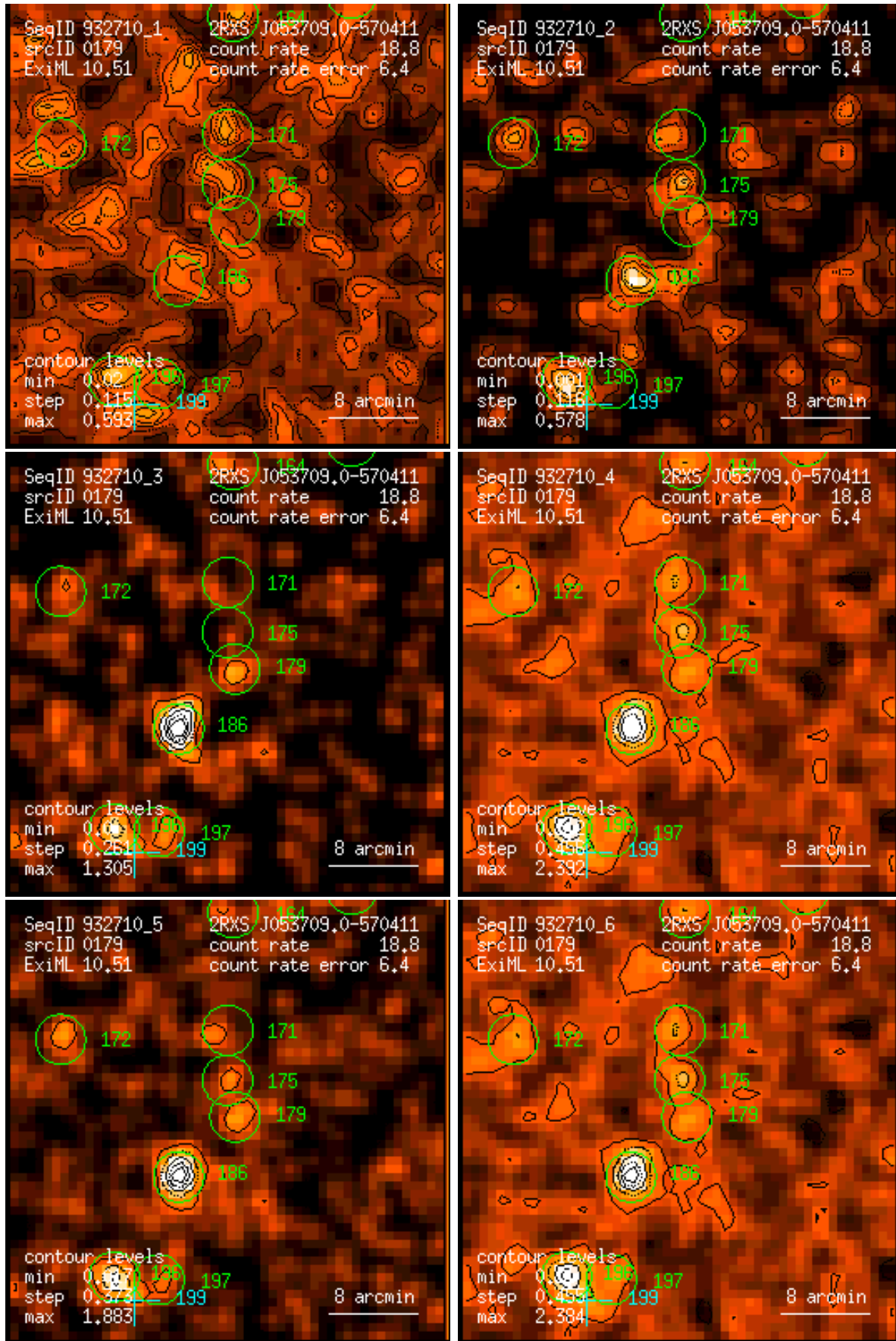
Figure 179: RASS 932710: detection 0179: band rate images, Gaussian filter: (1) PSPC channels 11 – 41, (2) 52 – 90, (3) 91 – 201, (4) 11 – 235, (5) 52 – 201, (6) 11 – 201. Broad band rates in counts/ks. Band rate contour levels in counts/ks/arcmin 2 .
