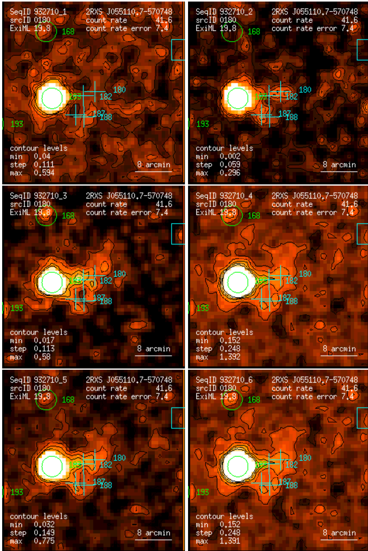
Figure 180: RASS 932710: detection 0180: band rate images, Gaussian filter: (1) PSPC channels 11 – 41, (2) 52 – 90, (3) 91 – 201, (4) 11 – 235, (5) 52 – 201, (6) 11 – 201. Broad band rates in counts/ks. Band rate contour levels in counts/ks/arcmin 2 .
