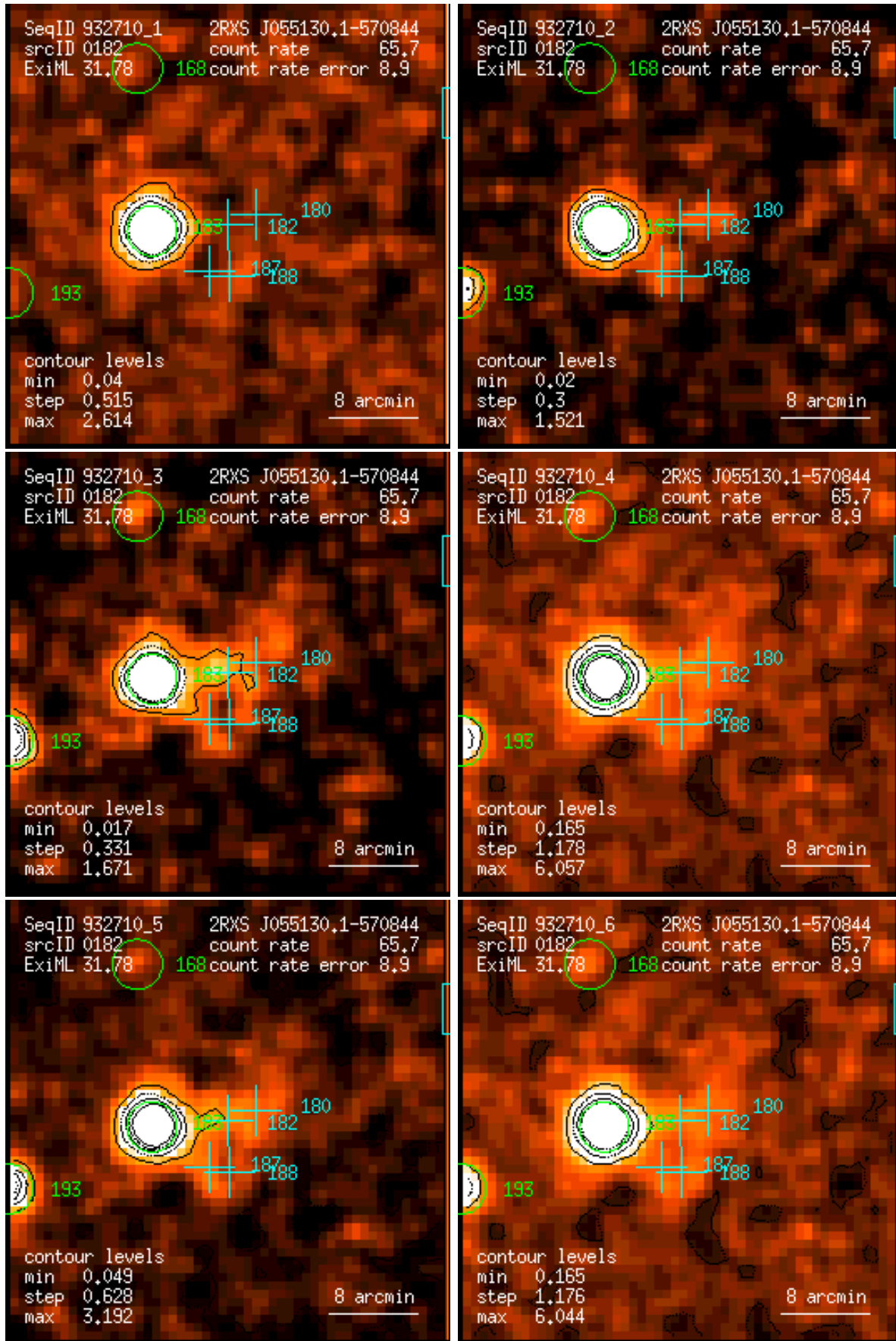
Figure 182: RASS 932710: detection 0182: band rate images, Gaussian filter: (1) PSPC channels 11 – 41, (2) 52 – 90, (3) 91 – 201, (4) 11 – 235, (5) 52 – 201, (6) 11 – 201. Broad band rates in counts/ks. Band rate contour levels in counts/ks/arcmin 2 .
