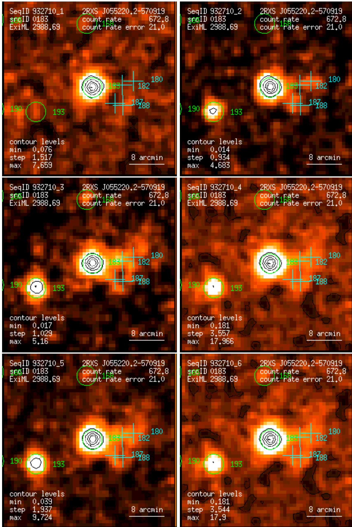
Figure 183: RASS 932710: detection 0183: band rate images, Gaussian filter: (1) PSPC channels 11 – 41, (2) 52 – 90, (3) 91 – 201, (4) 11 – 235, (5) 52 – 201, (6) 11 – 201. Broad band rates in counts/ks. Band rate contour levels in counts/ks/arcmin 2 .
