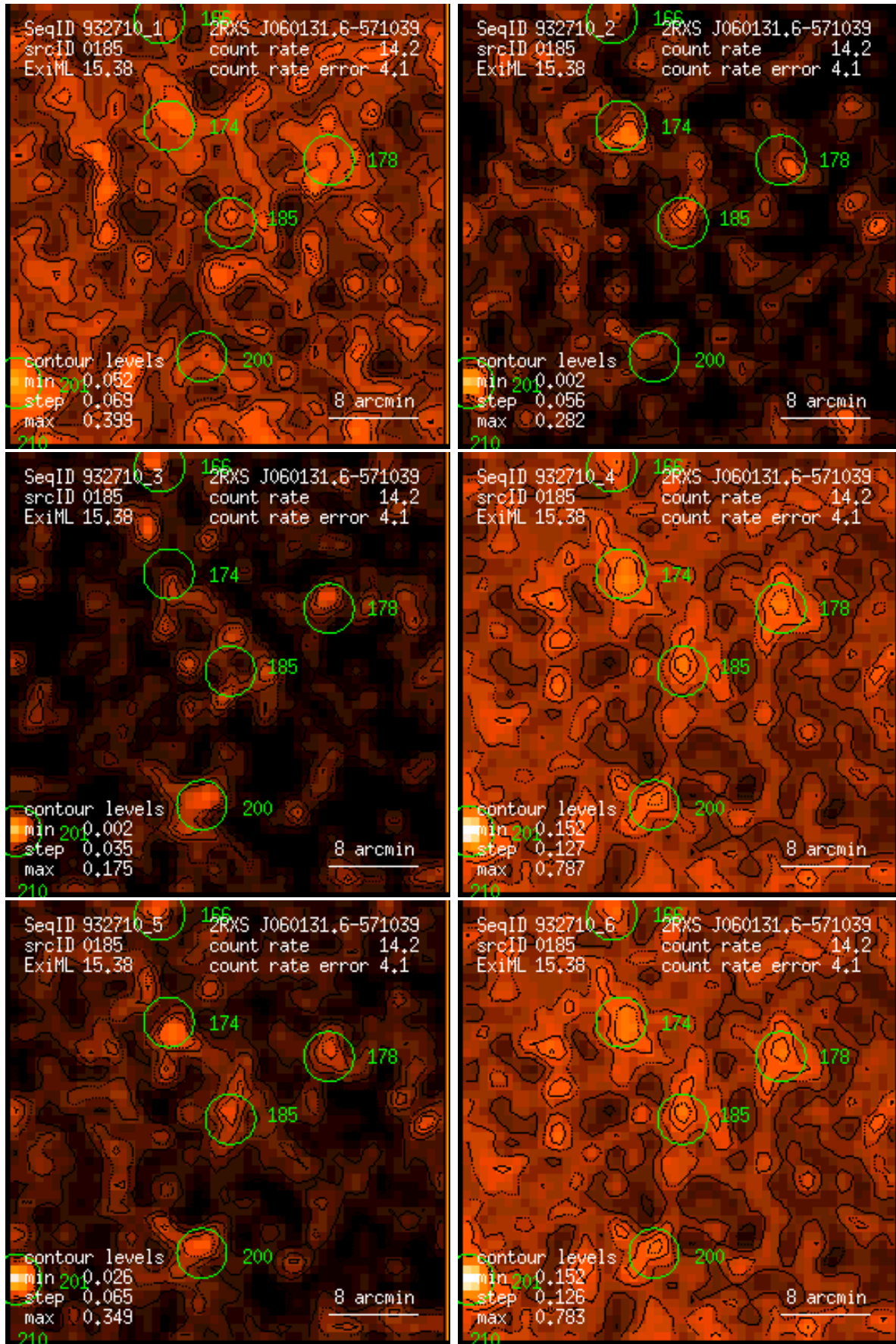
Figure 185: RASS 932710: detection 0185: band rate images, Gaussian filter: (1) PSPC channels 11 – 41, (2) 52 – 90, (3) 91 – 201, (4) 11 – 235, (5) 52 – 201, (6) 11 – 201. Broad band rates in counts/ks. Band rate contour levels in counts/ks/arcmin 2 .
