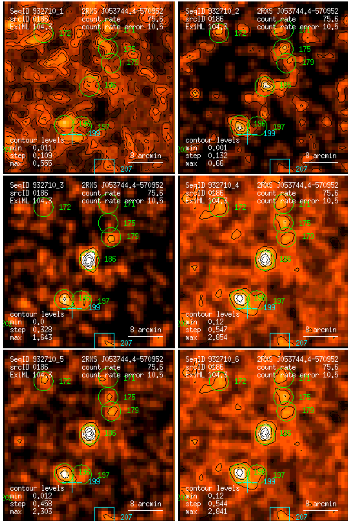
Figure 186: RASS 932710: detection 0186: band rate images, Gaussian filter: (1) PSPC channels 11 – 41, (2) 52 – 90, (3) 91 – 201, (4) 11 – 235, (5) 52 – 201, (6) 11 – 201. Broad band rates in counts/ks. Band rate contour levels in counts/ks/arcmin 2 .
