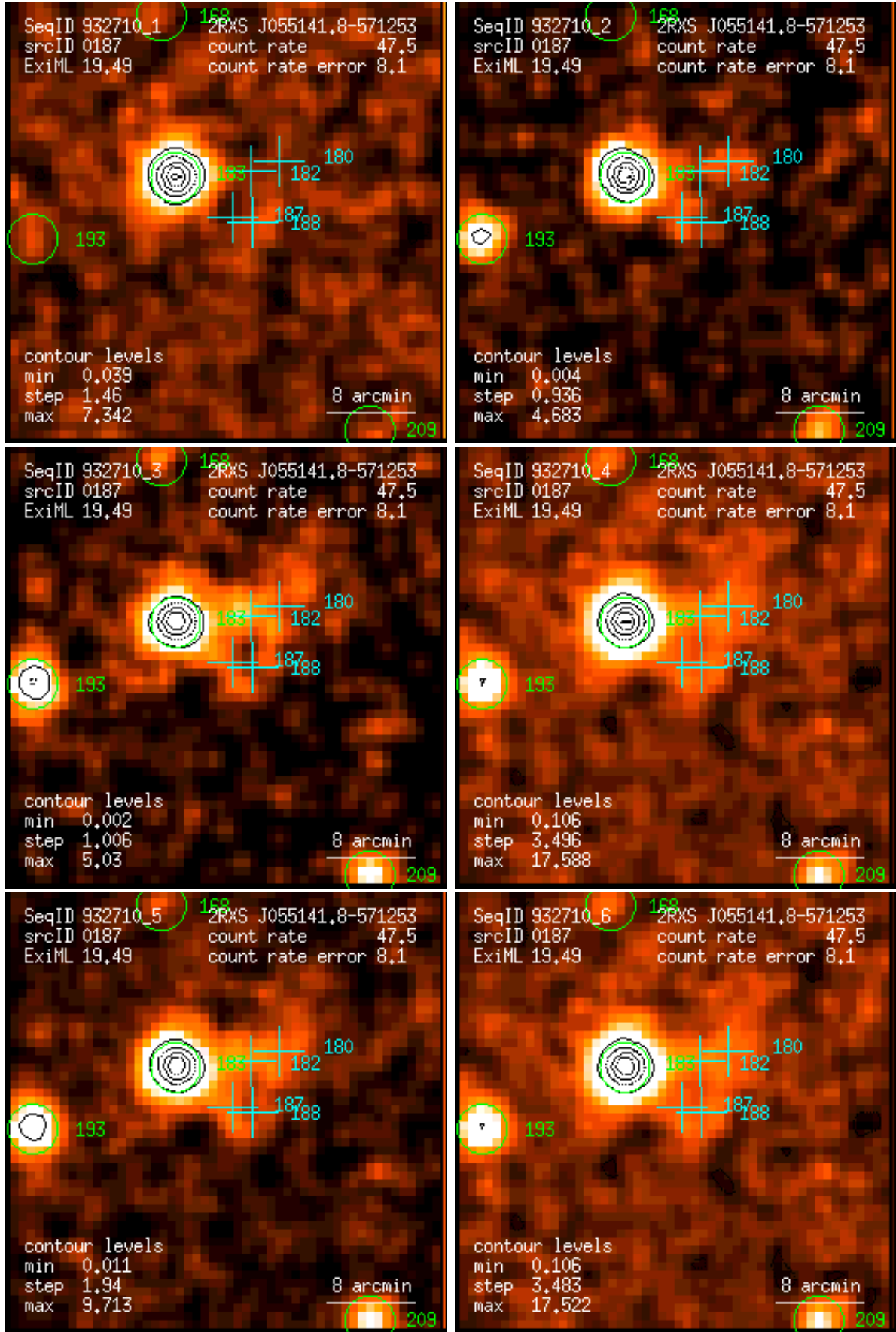
Figure 187: RASS 932710: detection 0187: band rate images, Gaussian filter: (1) PSPC channels 11 – 41, (2) 52 – 90, (3) 91 – 201, (4) 11 – 235, (5) 52 – 201, (6) 11 – 201. Broad band rates in counts/ks. Band rate contour levels in counts/ks/arcmin 2 .
