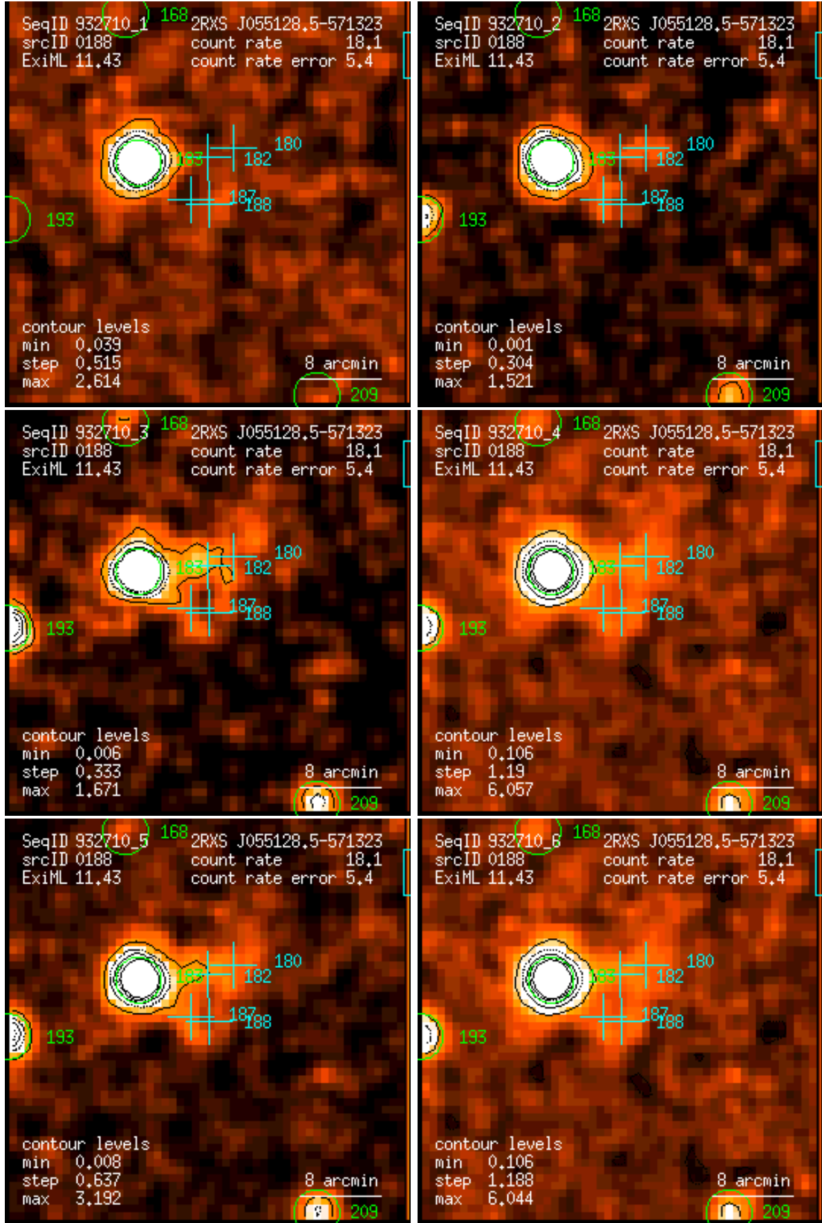
Figure 188: RASS 932710: detection 0188: band rate images, Gaussian filter: (1) PSPC channels 11 – 41, (2) 52 – 90, (3) 91 – 201, (4) 11 – 235, (5) 52 – 201, (6) 11 – 201. Broad band rates in counts/ks. Band rate contour levels in counts/ks/arcmin 2 .
