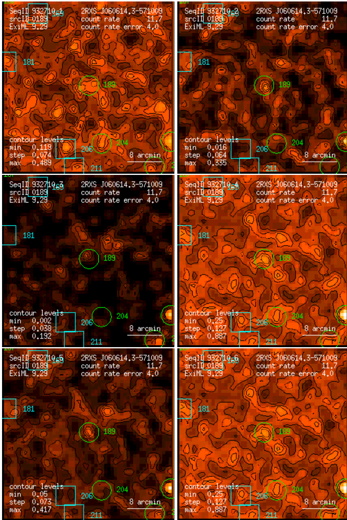
Figure 189: RASS 932710: detection 0189: band rate images, Gaussian filter: (1) PSPC channels 11 – 41, (2) 52 – 90, (3) 91 – 201, (4) 11 – 235, (5) 52 – 201, (6) 11 – 201. Broad band rates in counts/ks. Band rate contour levels in counts/ks/arcmin 2 .
