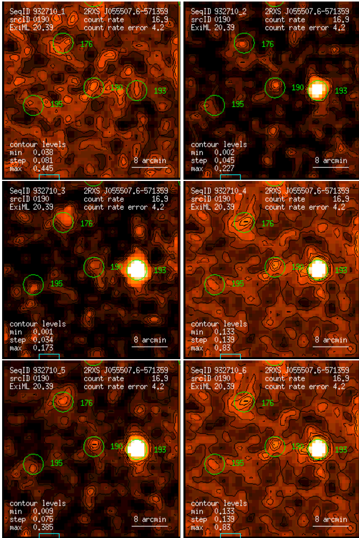
Figure 190: RASS 932710: detection 0190: band rate images, Gaussian filter: (1) PSPC channels 11 – 41, (2) 52 – 90, (3) 91 – 201, (4) 11 – 235, (5) 52 – 201, (6) 11 – 201. Broad band rates in counts/ks. Band rate contour levels in counts/ks/arcmin 2 .
