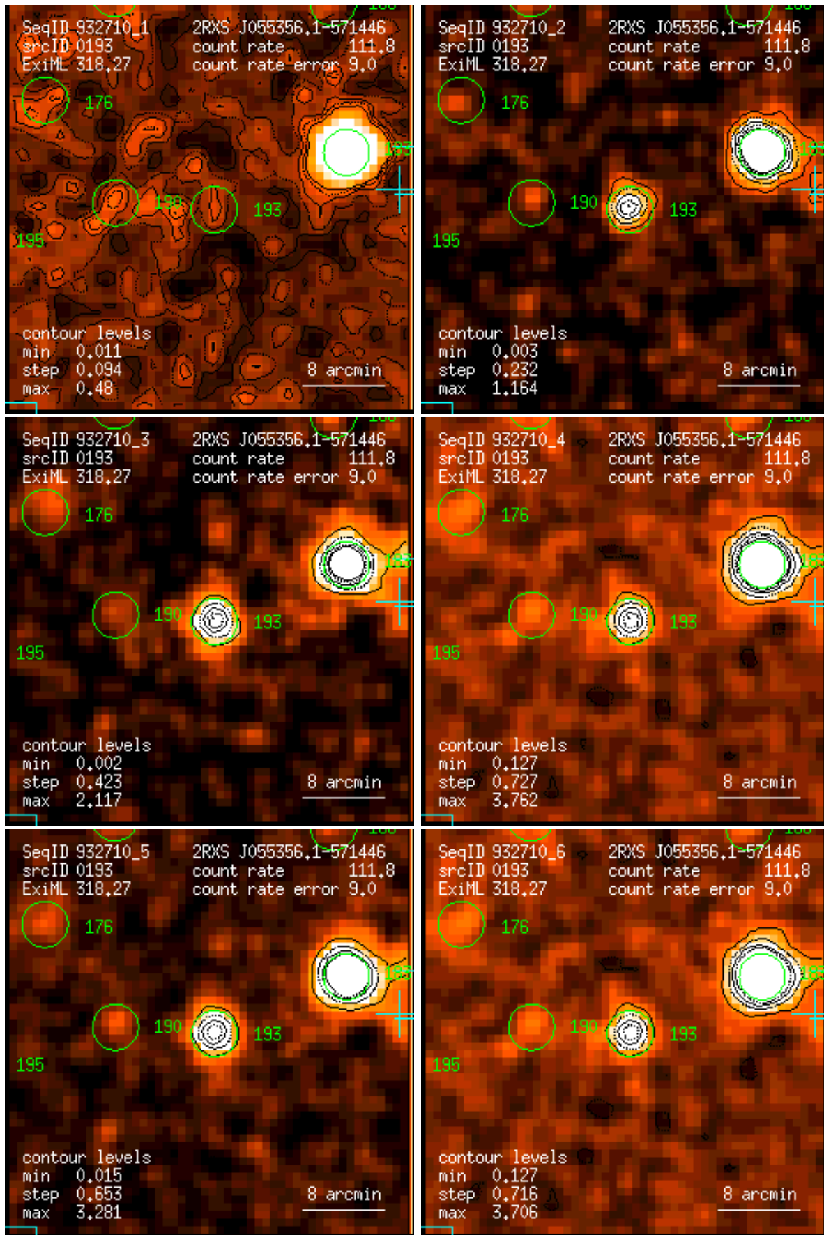
Figure 193: RASS 932710: detection 0193: band rate images, Gaussian filter: (1) PSPC channels 11 – 41, (2) 52 – 90, (3) 91 – 201, (4) 11 – 235, (5) 52 – 201, (6) 11 – 201. Broad band rates in counts/ks. Band rate contour levels in counts/ks/arcmin 2 .
