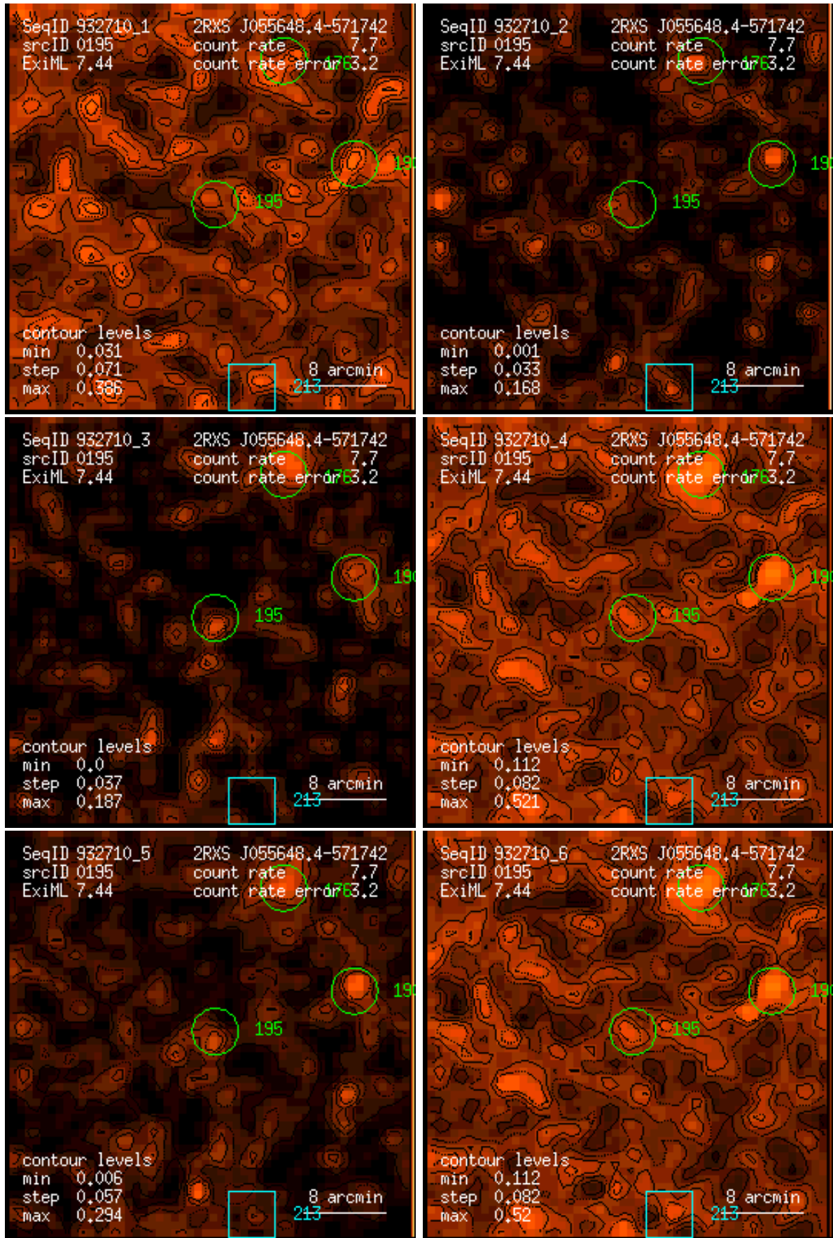
Figure 195: RASS 932710: detection 0195: band rate images, Gaussian filter: (1) PSPC channels 11 – 41, (2) 52 – 90, (3) 91 – 201, (4) 11 – 235, (5) 52 – 201, (6) 11 – 201. Broad band rates in counts/ks. Band rate contour levels in counts/ks/arcmin 2 .
