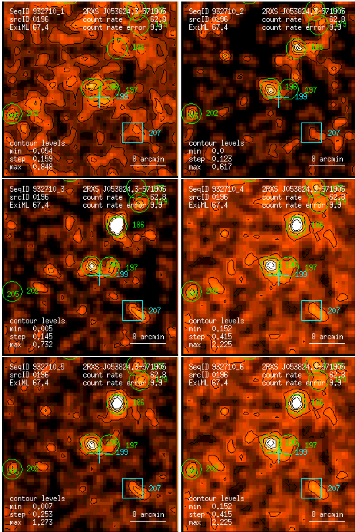
Figure 196: RASS 932710: detection 0196: band rate images, Gaussian filter: (1) PSPC channels 11 – 41, (2) 52 – 90, (3) 91 – 201, (4) 11 – 235, (5) 52 – 201, (6) 11 – 201. Broad band rates in counts/ks. Band rate contour levels in counts/ks/arcmin 2 .
