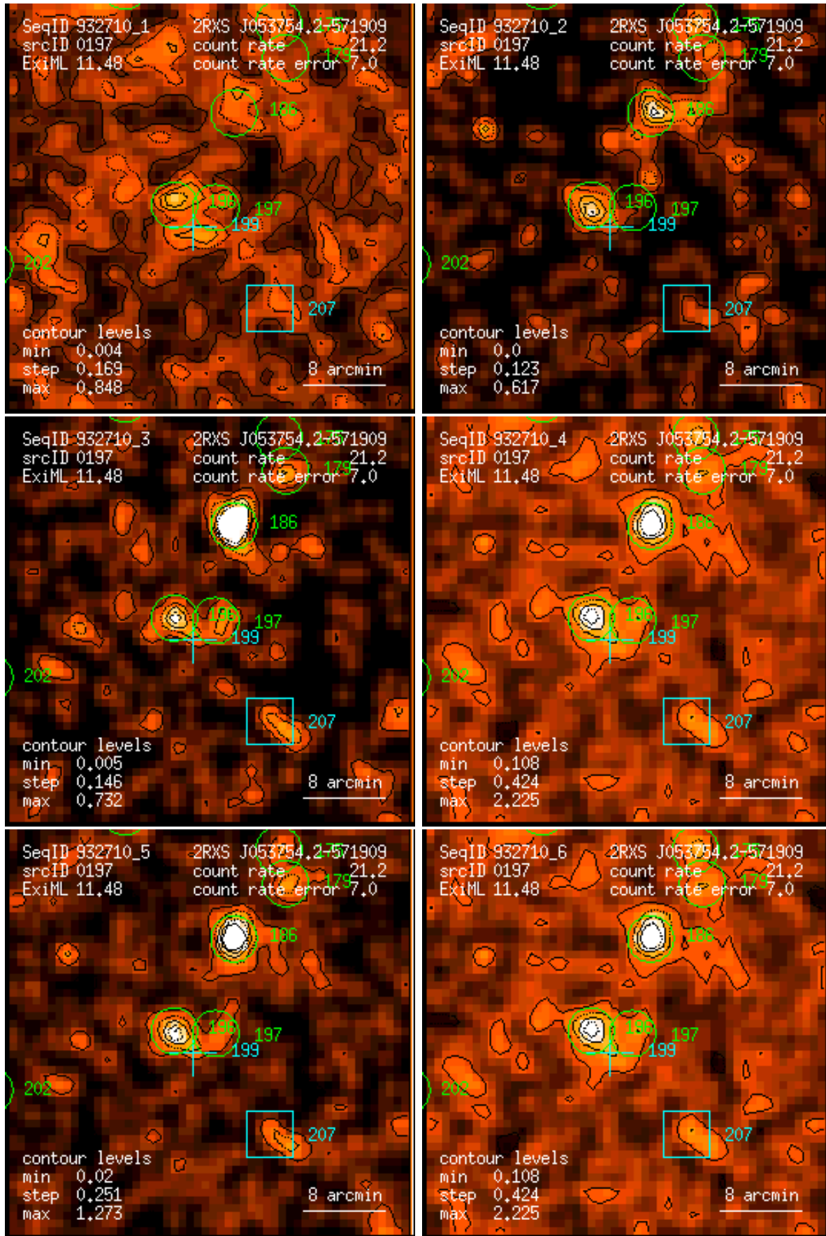
Figure 197: RASS 932710: detection 0197: band rate images, Gaussian filter: (1) PSPC channels 11 – 41, (2) 52 – 90, (3) 91 – 201, (4) 11 – 235, (5) 52 – 201, (6) 11 – 201. Broad band rates in counts/ks. Band rate contour levels in counts/ks/arcmin 2 .
