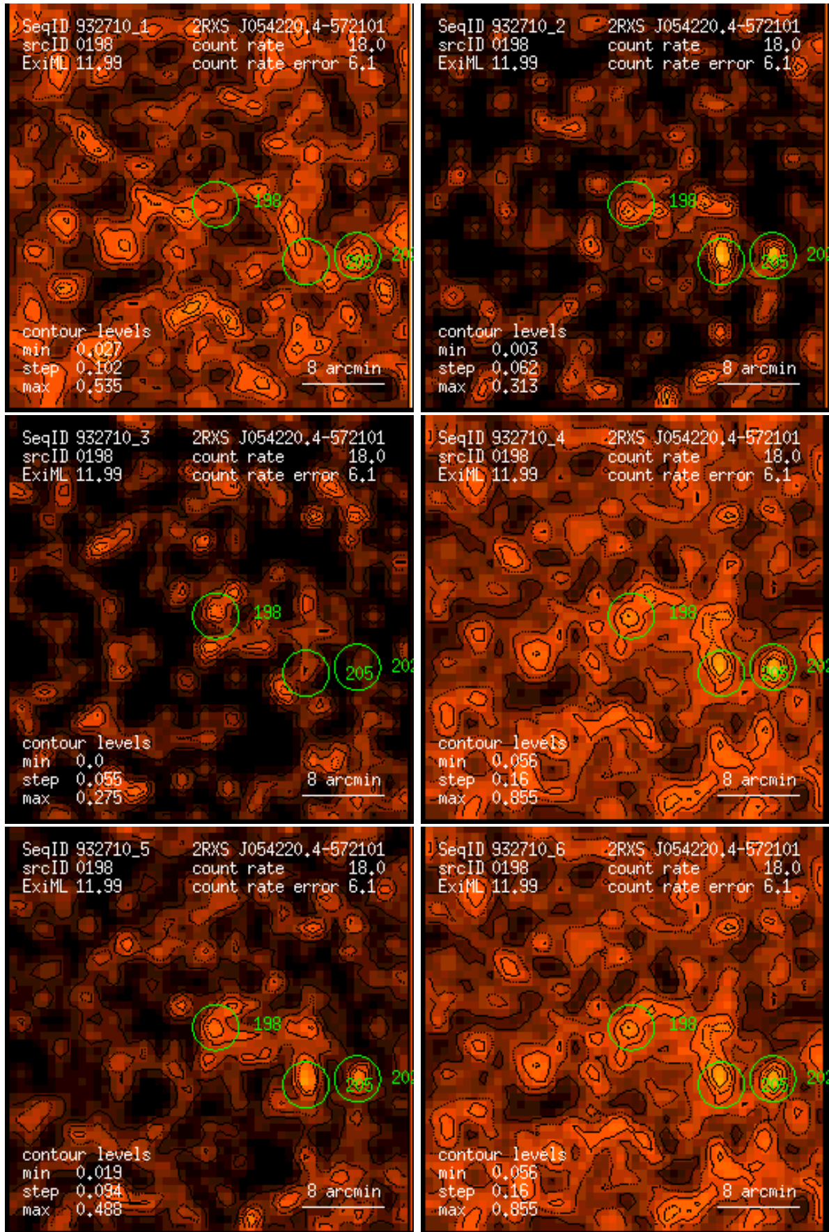
Figure 198: RASS 932710: detection 0198: band rate images, Gaussian filter: (1) PSPC channels 11 – 41, (2) 52 – 90, (3) 91 – 201, (4) 11 – 235, (5) 52 – 201, (6) 11 – 201. Broad band rates in counts/ks. Band rate contour levels in counts/ks/arcmin 2 .
