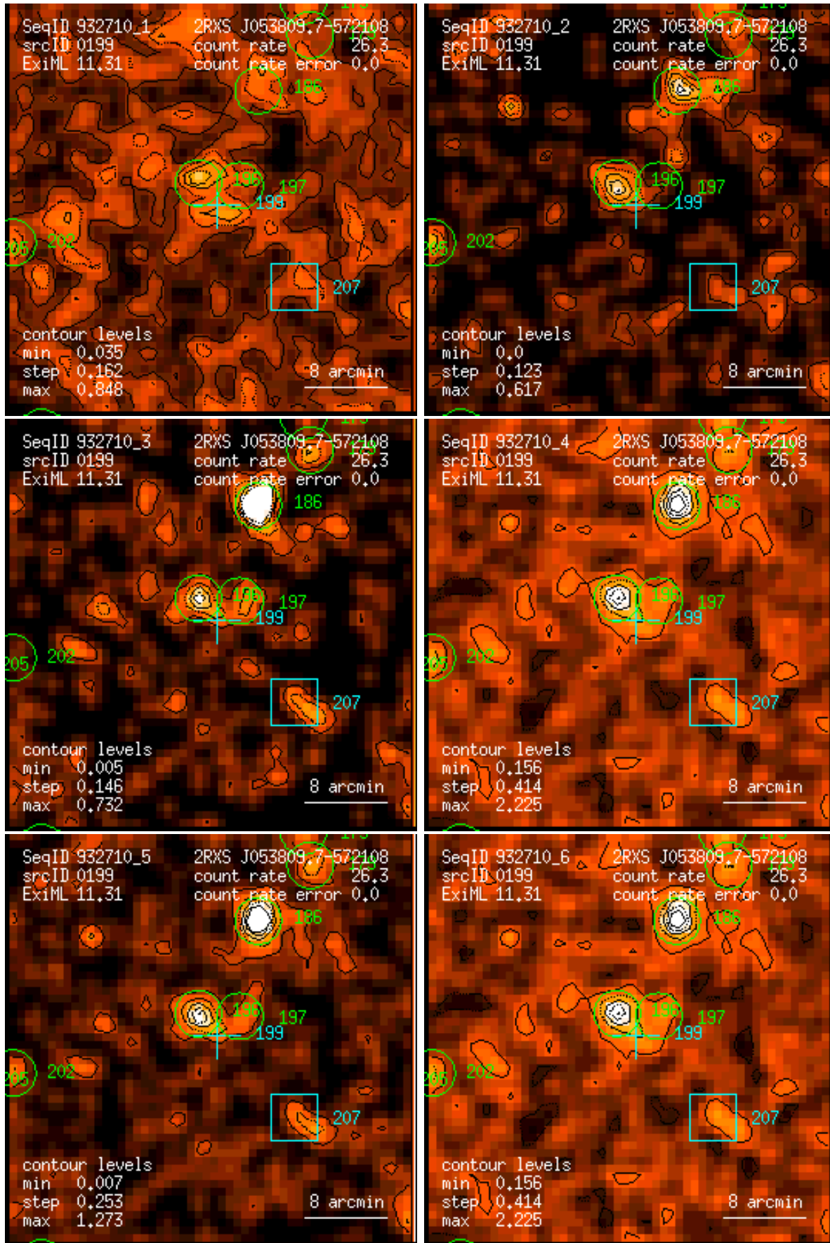
Figure 199: RASS 932710: detection 0199: band rate images, Gaussian filter: (1) PSPC channels 11 – 41, (2) 52 – 90, (3) 91 – 201, (4) 11 – 235, (5) 52 – 201, (6) 11 – 201. Broad band rates in counts/ks. Band rate contour levels in counts/ks/arcmin 2 .
