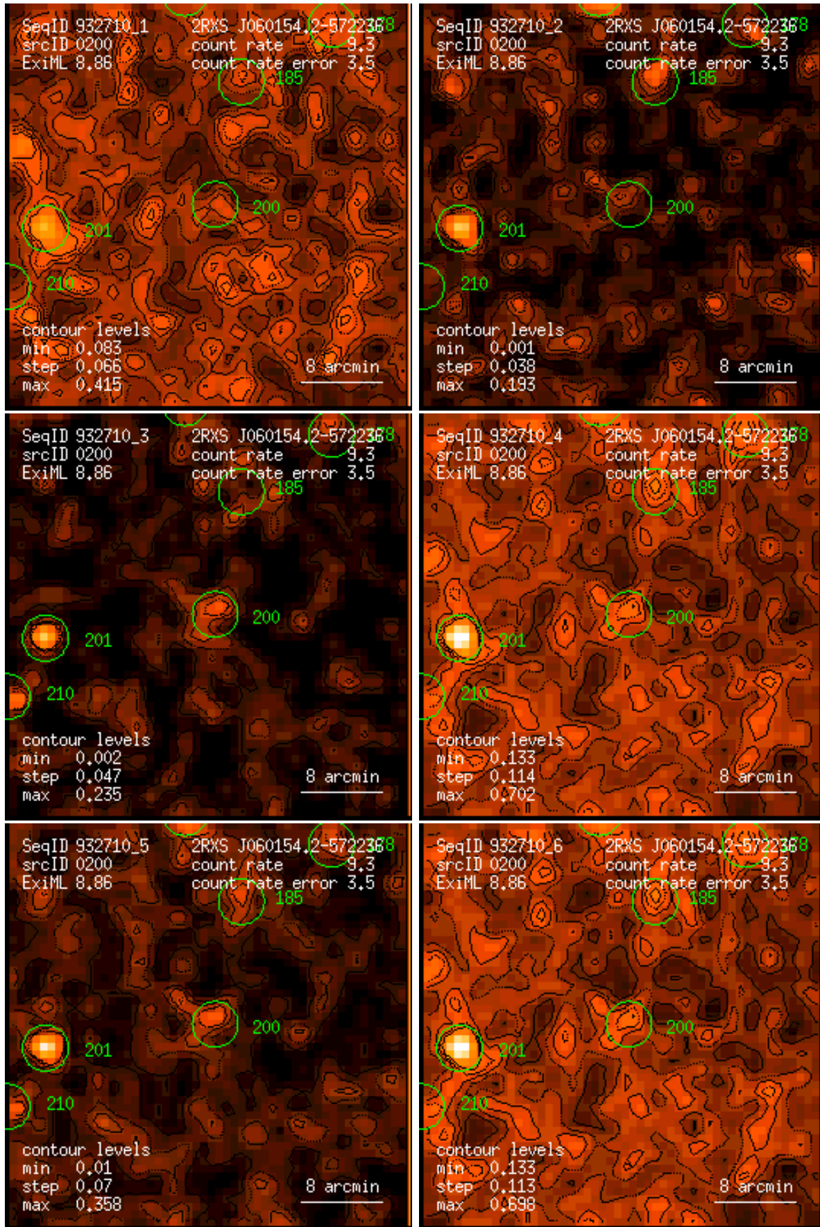
Figure 200: RASS 932710: detection 0200: band rate images, Gaussian filter: (1) PSPC channels 11 – 41, (2) 52 – 90, (3) 91 – 201, (4) 11 – 235, (5) 52 – 201, (6) 11 – 201. Broad band rates in counts/ks. Band rate contour levels in counts/ks/arcmin 2 .
