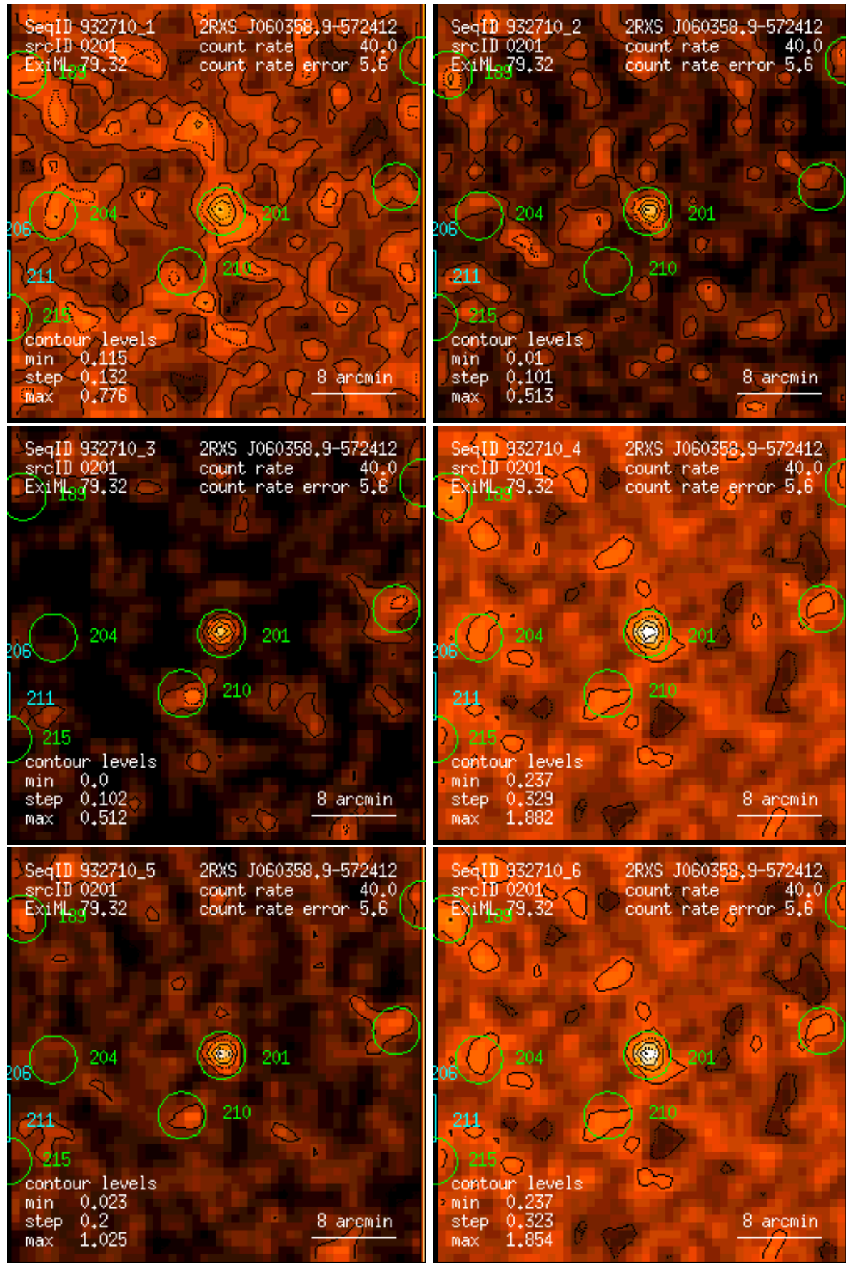
Figure 201: RASS 932710: detection 0201: band rate images, Gaussian filter: (1) PSPC channels 11 – 41, (2) 52 – 90, (3) 91 – 201, (4) 11 – 235, (5) 52 – 201, (6) 11 – 201. Broad band rates in counts/ks. Band rate contour levels in counts/ks/arcmin 2 .
