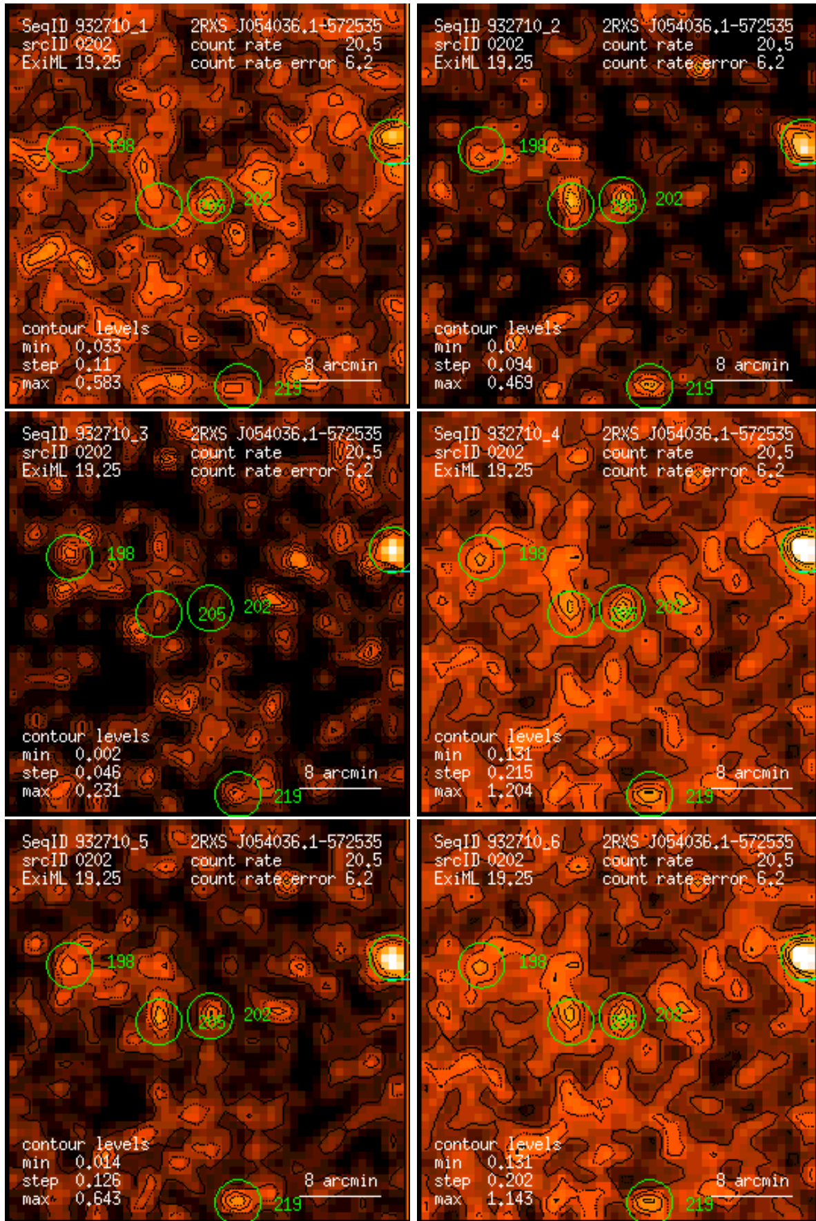
Figure 202: RASS 932710: detection 0202: band rate images, Gaussian filter: (1) PSPC channels 11 – 41, (2) 52 – 90, (3) 91 – 201, (4) 11 – 235, (5) 52 – 201, (6) 11 – 201. Broad band rates in counts/ks. Band rate contour levels in counts/ks/arcmin 2 .
