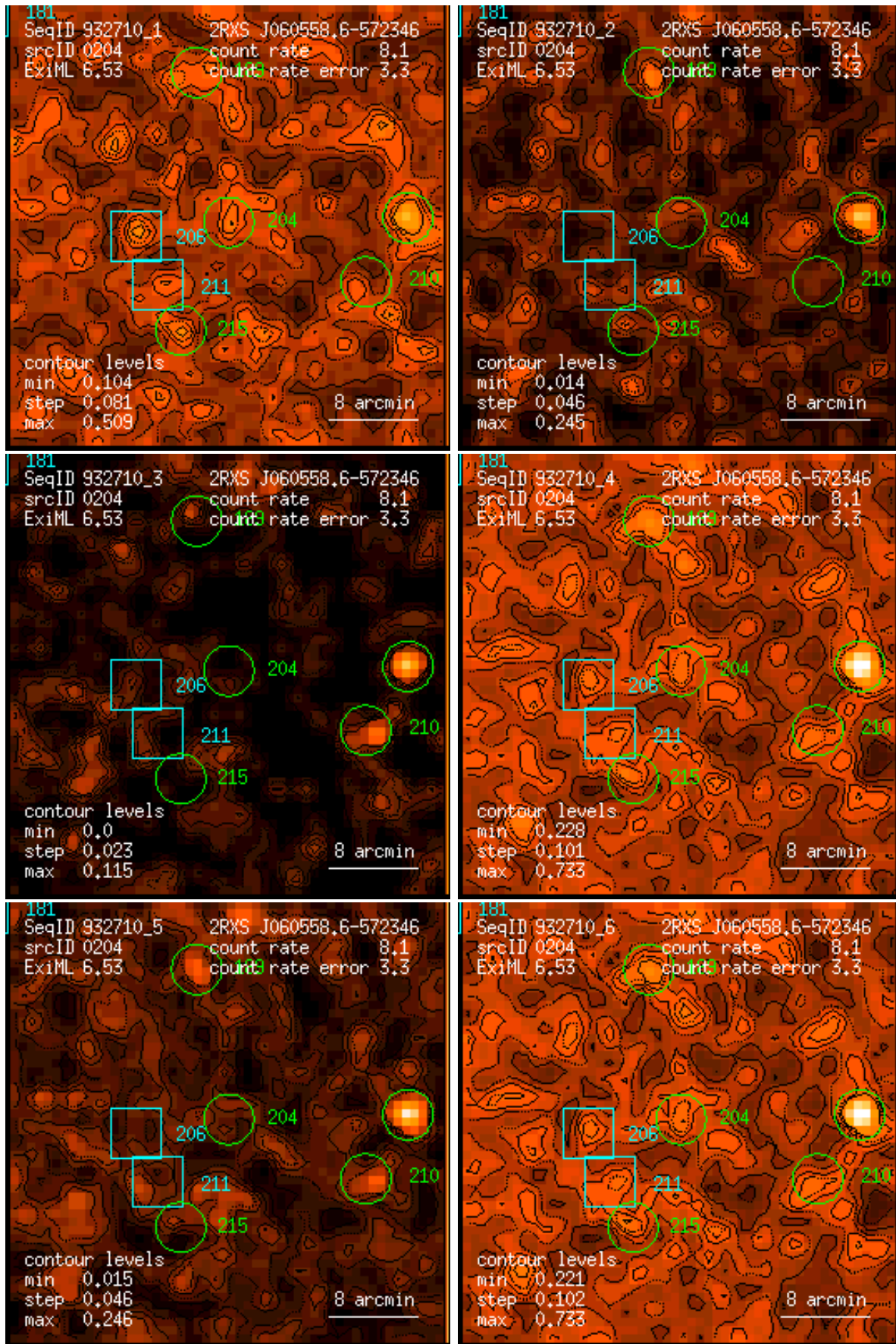
Figure 204: RASS 932710: detection 0204: band rate images, Gaussian filter: (1) PSPC channels 11 – 41, (2) 52 – 90, (3) 91 – 201, (4) 11 – 235, (5) 52 – 201, (6) 11 – 201. Broad band rates in counts/ks. Band rate contour levels in counts/ks/arcmin 2 .
