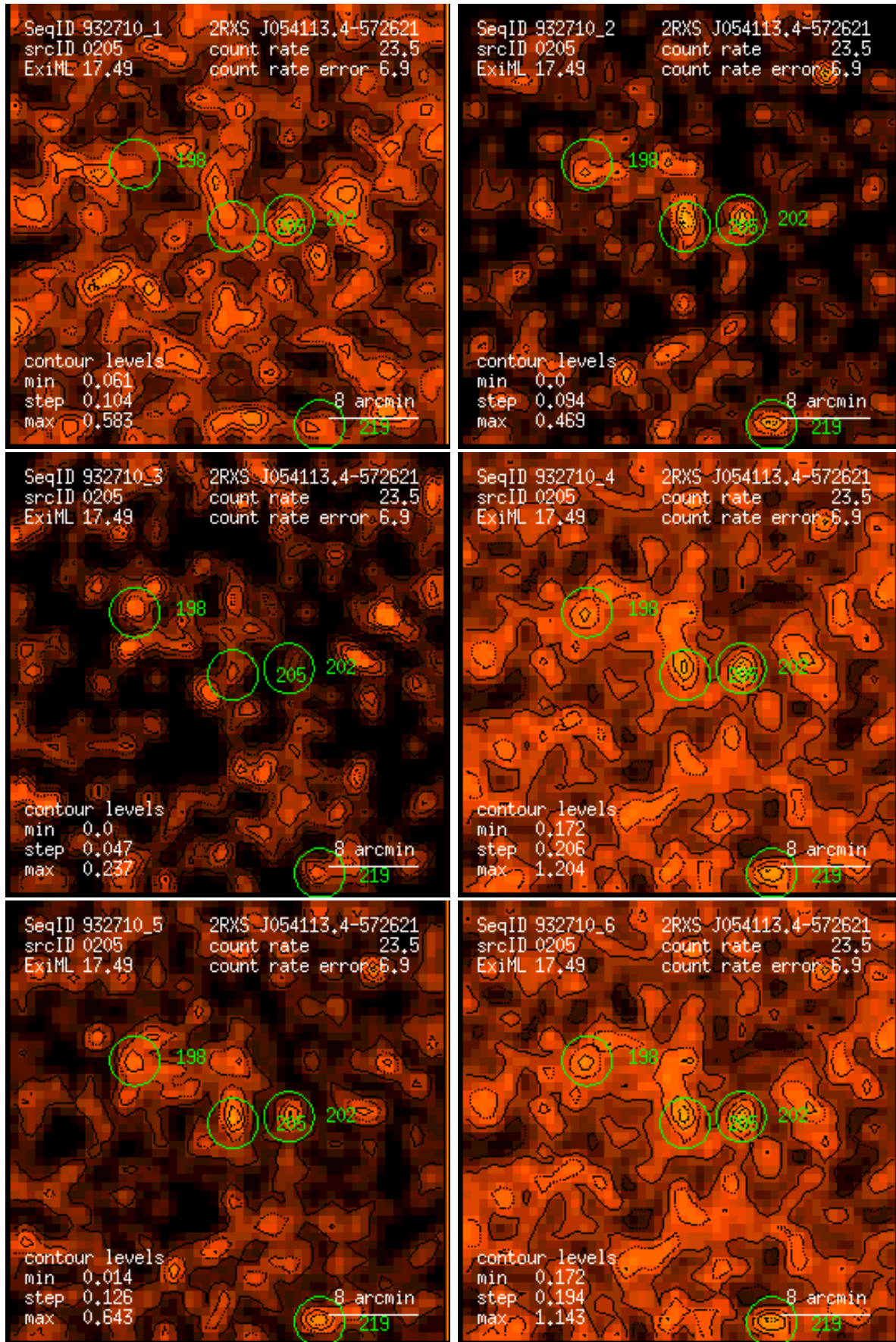
Figure 205: RASS 932710: detection 0205: band rate images, Gaussian filter: (1) PSPC channels 11 – 41, (2) 52 – 90, (3) 91 – 201, (4) 11 – 235, (5) 52 – 201, (6) 11 – 201. Broad band rates in counts/ks. Band rate contour levels in counts/ks/arcmin 2 .
