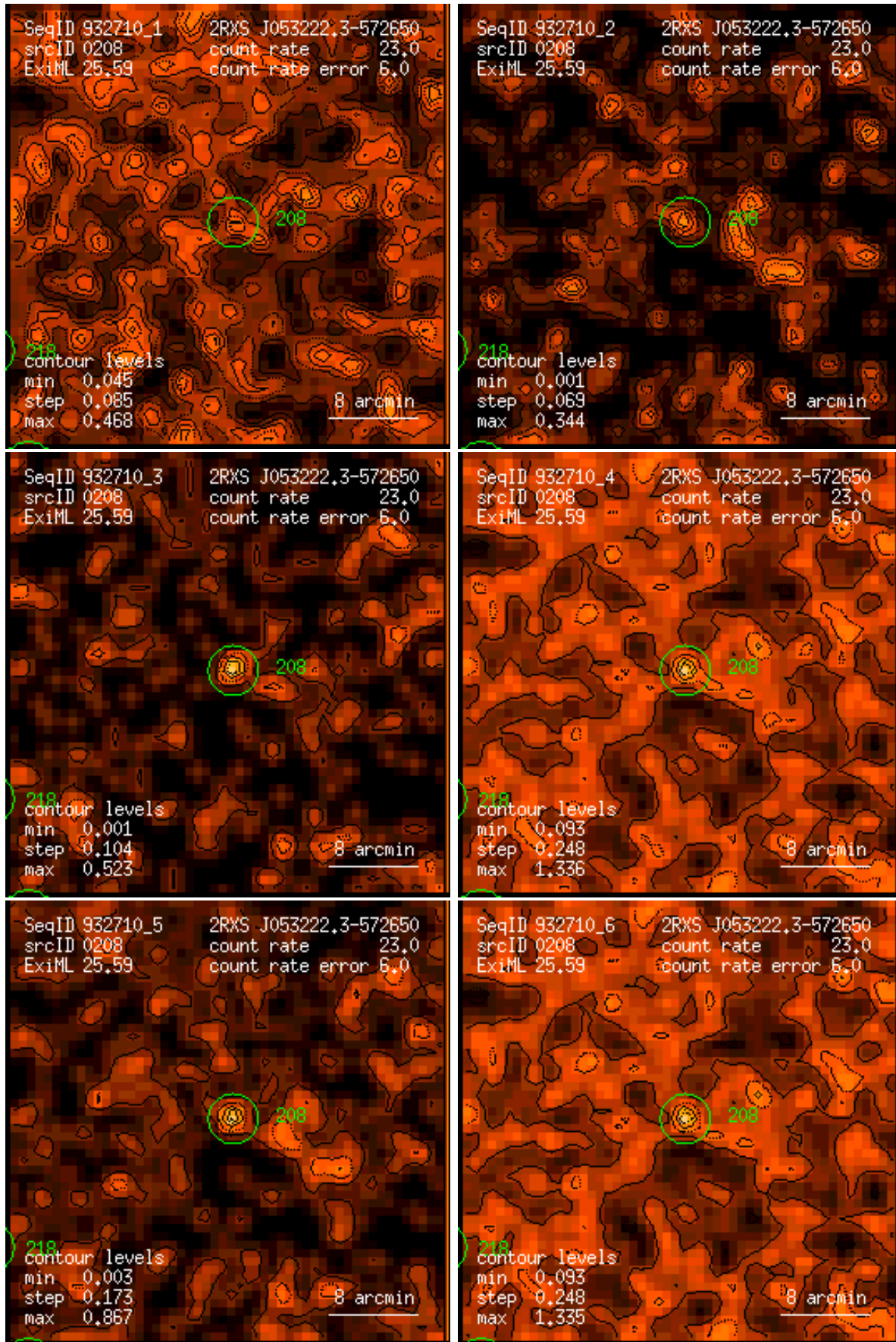
Figure 208: RASS 932710: detection 0208: band rate images, Gaussian filter: (1) PSPC channels 11 – 41, (2) 52 – 90, (3) 91 – 201, (4) 11 – 235, (5) 52 – 201, (6) 11 – 201. Broad band rates in counts/ks. Band rate contour levels in counts/ks/arcmin 2 .
