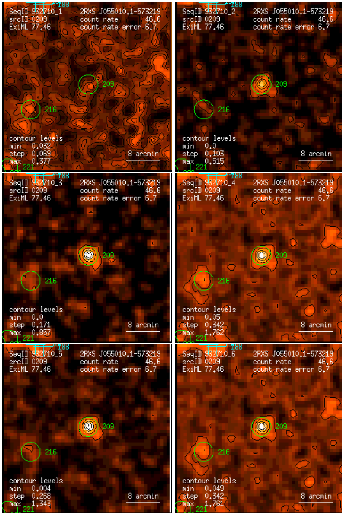
Figure 209: RASS 932710: detection 0209: band rate images, Gaussian filter: (1) PSPC channels 11 – 41, (2) 52 – 90, (3) 91 – 201, (4) 11 – 235, (5) 52 – 201, (6) 11 – 201. Broad band rates in counts/ks. Band rate contour levels in counts/ks/arcmin 2 .
