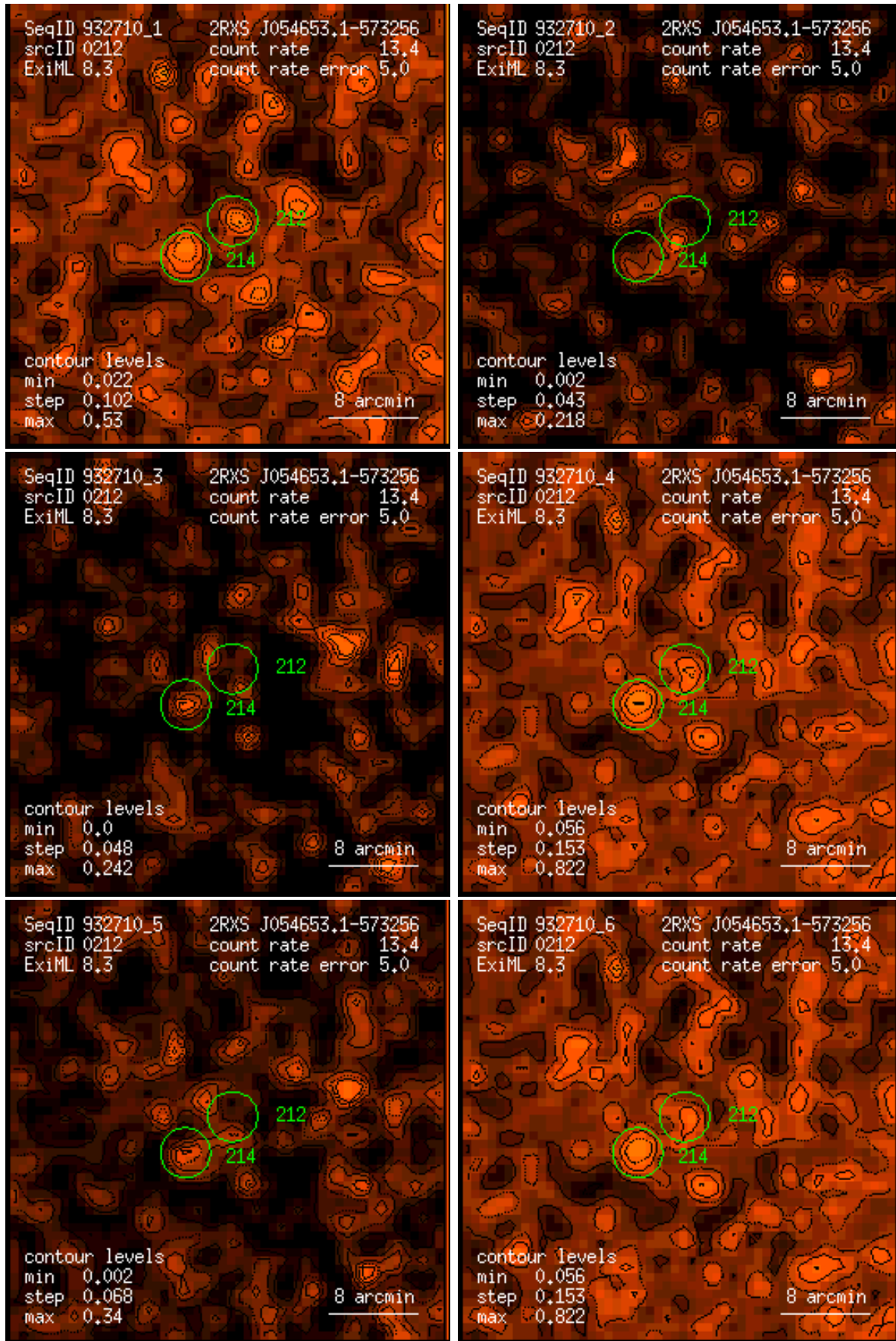
Figure 212: RASS 932710: detection 0212: band rate images, Gaussian filter: (1) PSPC channels 11 – 41, (2) 52 – 90, (3) 91 – 201, (4) 11 – 235, (5) 52 – 201, (6) 11 – 201. Broad band rates in counts/ks. Band rate contour levels in counts/ks/arcmin 2 .
