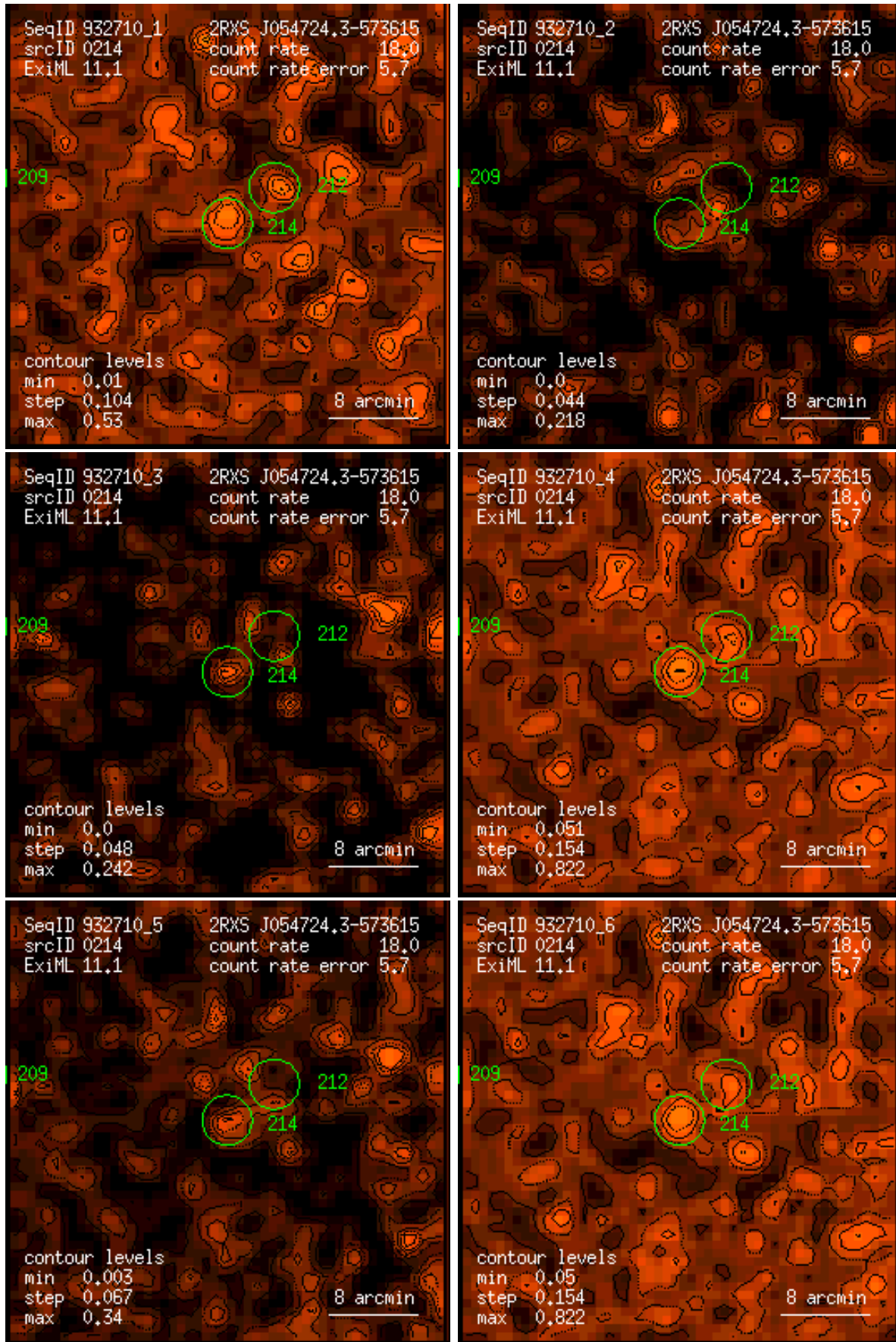
Figure 214: RASS 932710: detection 0214: band rate images, Gaussian filter: (1) PSPC channels 11 – 41, (2) 52 – 90, (3) 91 – 201, (4) 11 – 235, (5) 52 – 201, (6) 11 – 201. Broad band rates in counts/ks. Band rate contour levels in counts/ks/arcmin 2 .
