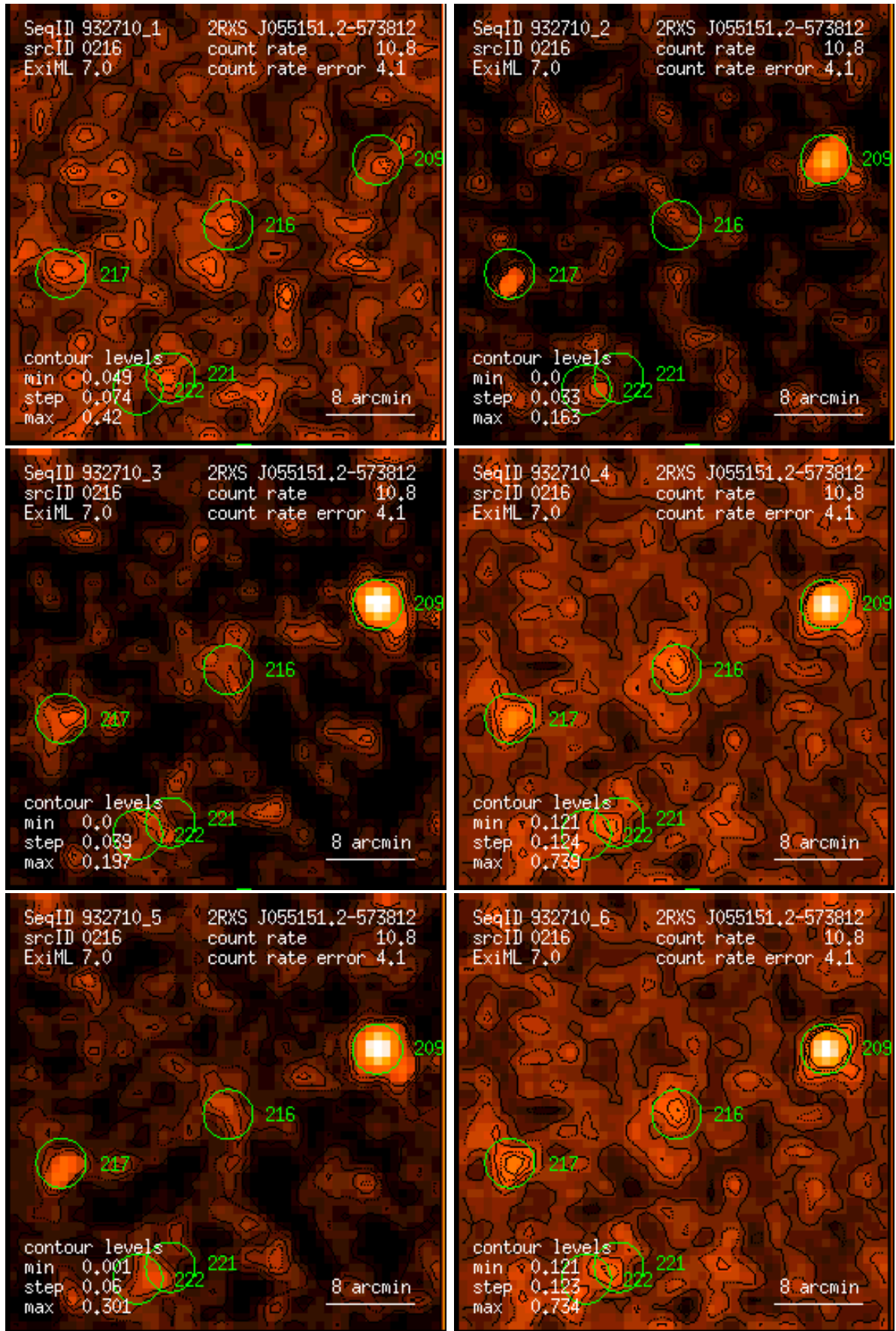
Figure 216: RASS 932710: detection 0216: band rate images, Gaussian filter: (1) PSPC channels 11 – 41, (2) 52 – 90, (3) 91 – 201, (4) 11 – 235, (5) 52 – 201, (6) 11 – 201. Broad band rates in counts/ks. Band rate contour levels in counts/ks/arcmin 2 .
