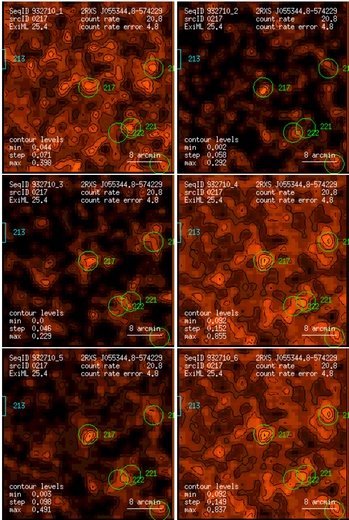
Figure 217: RASS 932710: detection 0217: band rate images, Gaussian filter: (1) PSPC channels 11 – 41, (2) 52 – 90, (3) 91 – 201, (4) 11 – 235, (5) 52 – 201, (6) 11 – 201. Broad band rates in counts/ks. Band rate contour levels in counts/ks/arcmin 2 .
