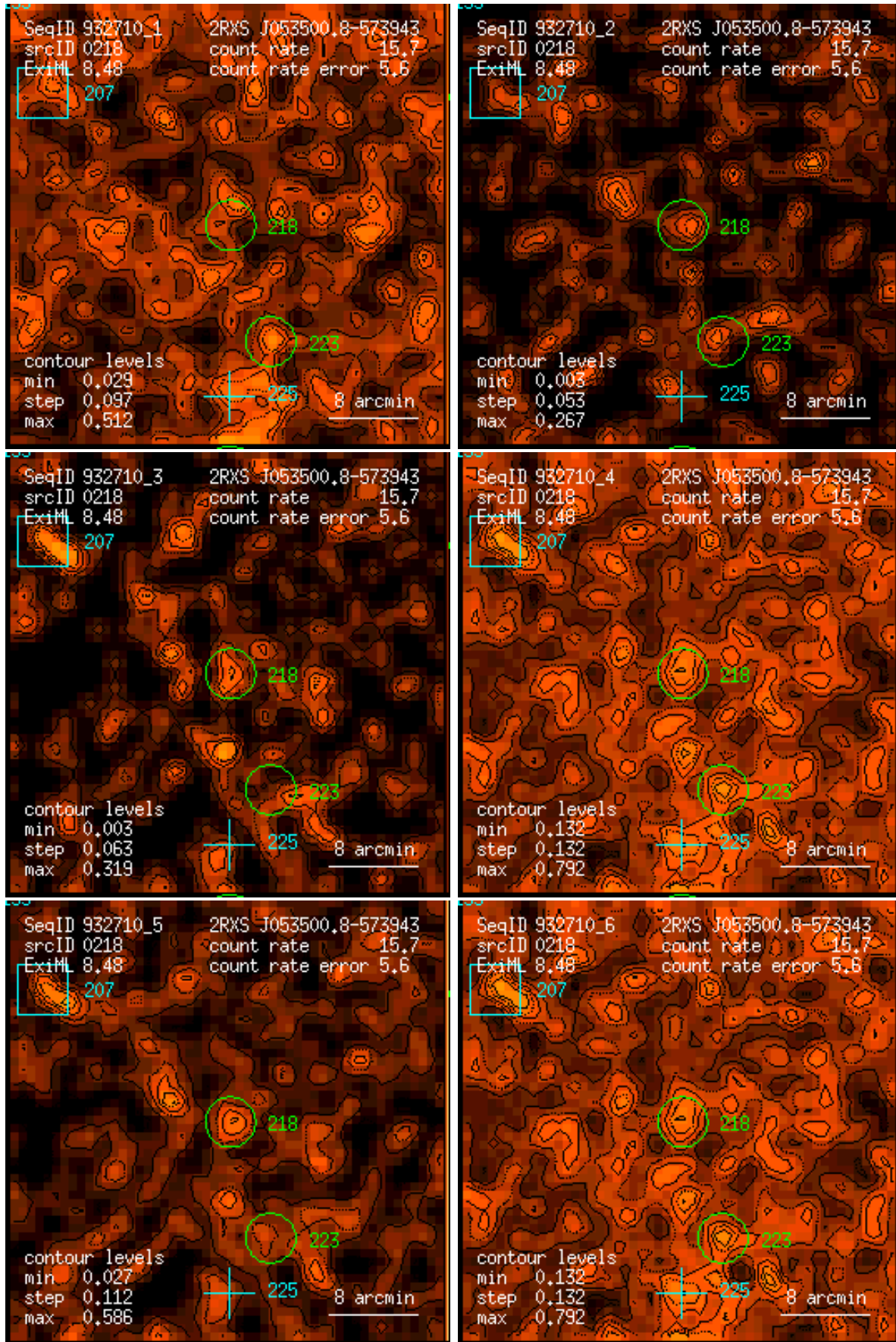
Figure 218: RASS 932710: detection 0218: band rate images, Gaussian filter: (1) PSPC channels 11 – 41, (2) 52 – 90, (3) 91 – 201, (4) 11 – 235, (5) 52 – 201, (6) 11 – 201. Broad band rates in counts/ks. Band rate contour levels in counts/ks/arcmin 2 .
