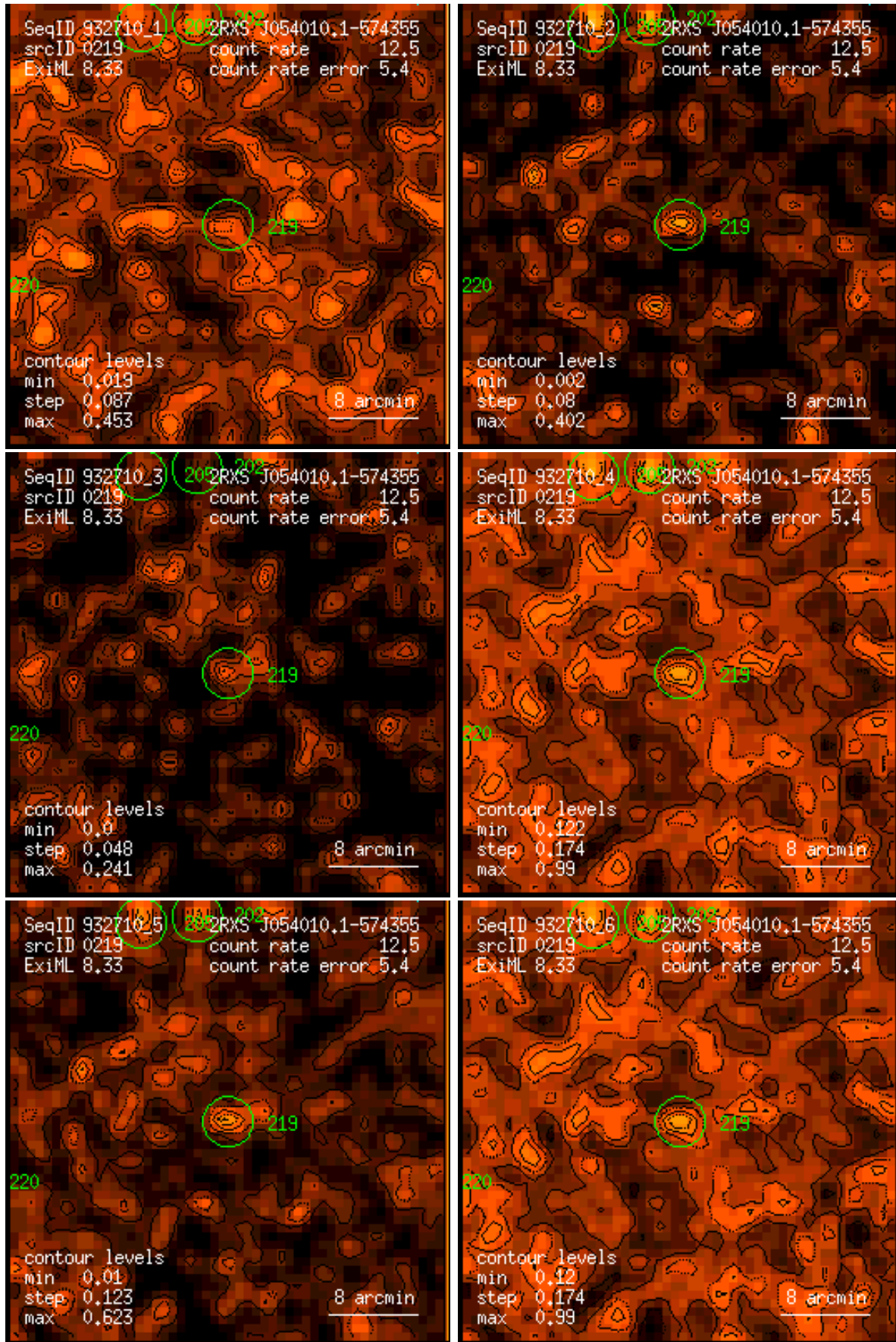
Figure 219: RASS 932710: detection 0219: band rate images, Gaussian filter: (1) PSPC channels 11 – 41, (2) 52 – 90, (3) 91 – 201, (4) 11 – 235, (5) 52 – 201, (6) 11 – 201. Broad band rates in counts/ks. Band rate contour levels in counts/ks/arcmin 2 .
