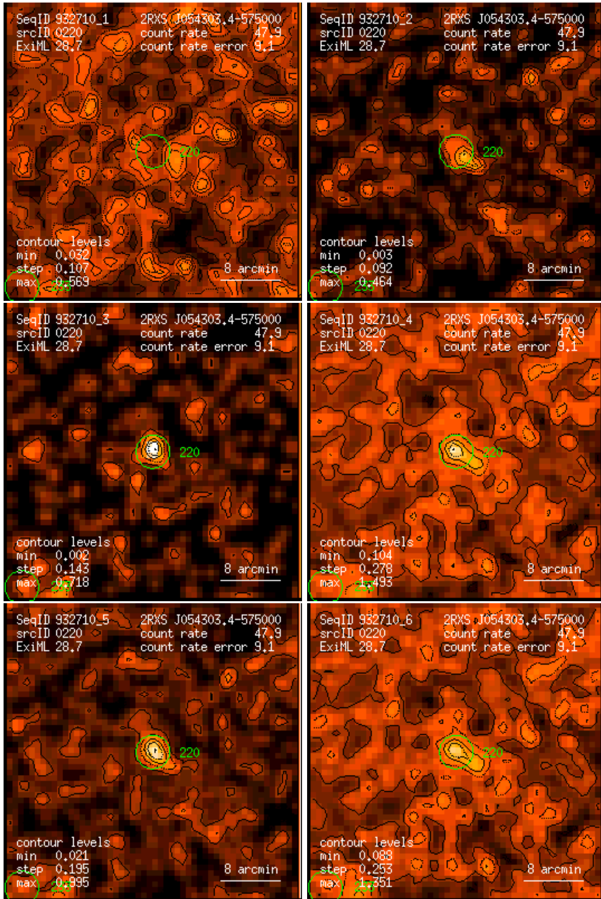
Figure 220: RASS 932710: detection 0220: band rate images, Gaussian filter: (1) PSPC channels 11 – 41, (2) 52 – 90, (3) 91 – 201, (4) 11 – 235, (5) 52 – 201, (6) 11 – 201. Broad band rates in counts/ks. Band rate contour levels in counts/ks/arcmin 2 .
