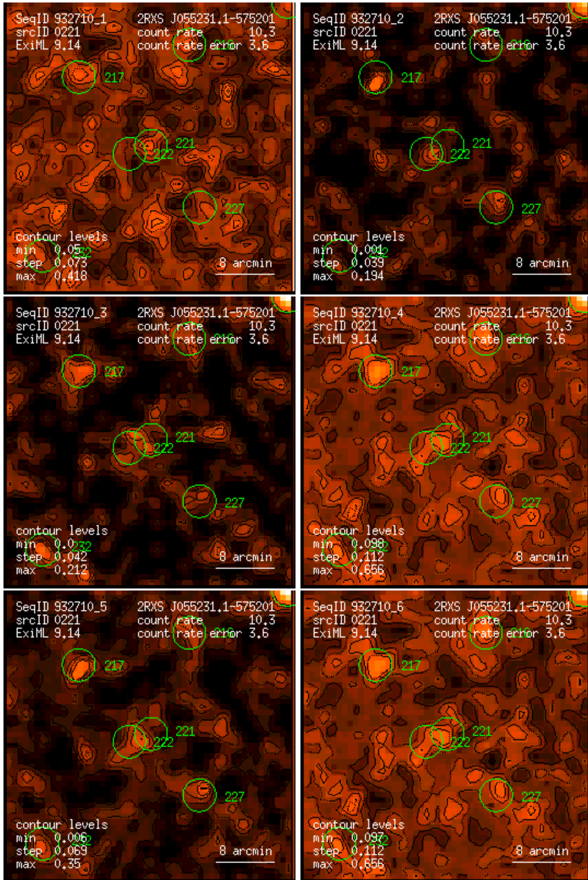
Figure 221: RASS 932710: detection 0221: band rate images, Gaussian filter: (1) PSPC channels 11 – 41, (2) 52 – 90, (3) 91 – 201, (4) 11 – 235, (5) 52 – 201, (6) 11 – 201. Broad band rates in counts/ks. Band rate contour levels in counts/ks/arcmin 2 .
