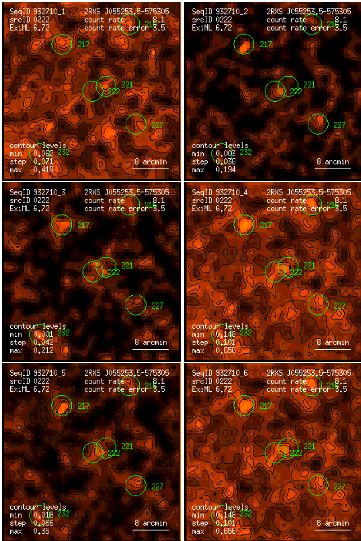
Figure 222: RASS 932710: detection 0222: band rate images, Gaussian filter: (1) PSPC channels 11 – 41, (2) 52 – 90, (3) 91 – 201, (4) 11 – 235, (5) 52 – 201, (6) 11 – 201. Broad band rates in counts/ks. Band rate contour levels in counts/ks/arcmin 2 .
