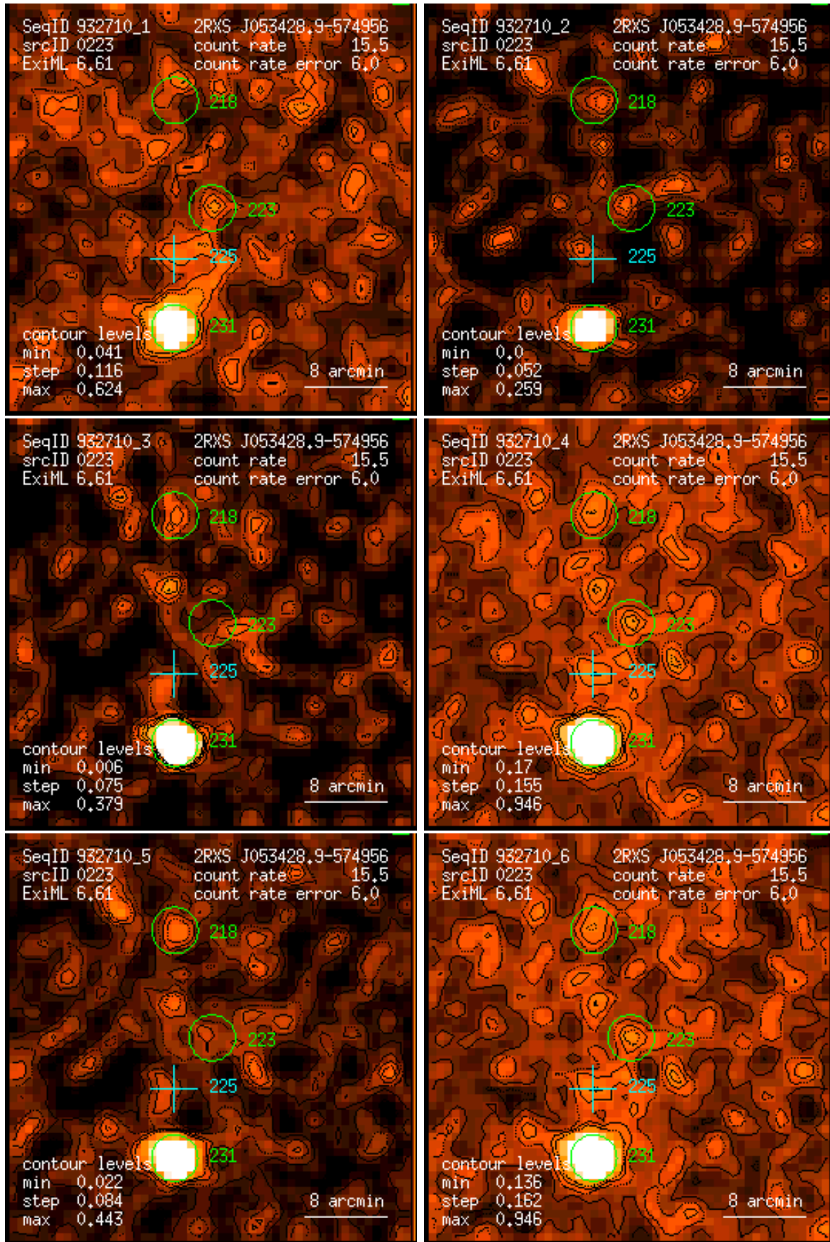
Figure 223: RASS 932710: detection 0223: band rate images, Gaussian filter: (1) PSPC channels 11 – 41, (2) 52 – 90, (3) 91 – 201, (4) 11 – 235, (5) 52 – 201, (6) 11 – 201. Broad band rates in counts/ks. Band rate contour levels in counts/ks/arcmin 2 .
