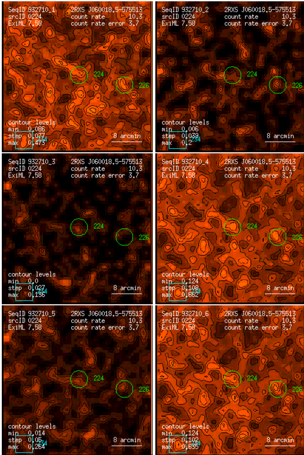
Figure 224: RASS 932710: detection 0224: band rate images, Gaussian filter: (1) PSPC channels 11 – 41, (2) 52 – 90, (3) 91 – 201, (4) 11 – 235, (5) 52 – 201, (6) 11 – 201. Broad band rates in counts/ks. Band rate contour levels in counts/ks/arcmin 2 .
