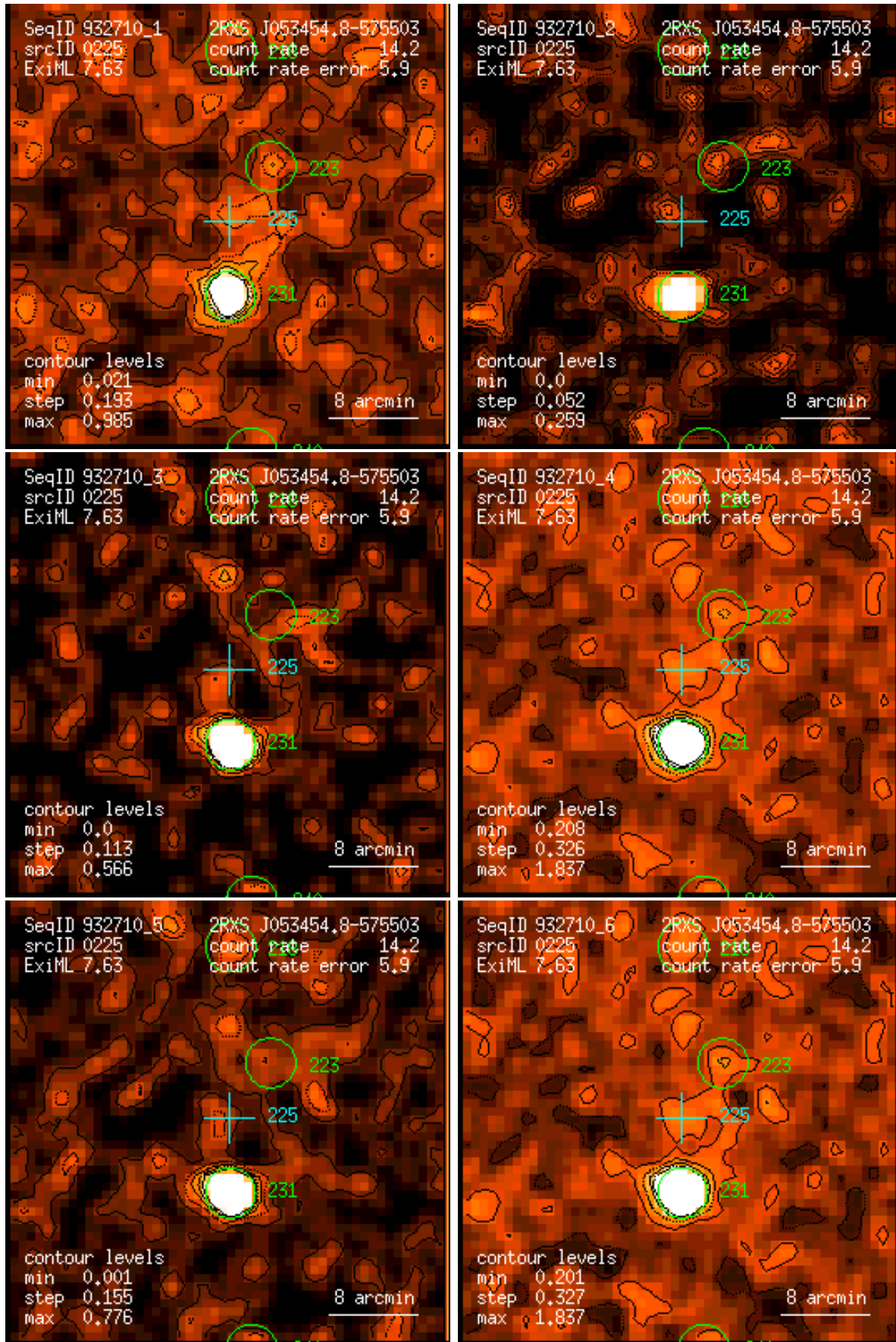
Figure 225: RASS 932710: detection 0225: band rate images, Gaussian filter: (1) PSPC channels 11 – 41, (2) 52 – 90, (3) 91 – 201, (4) 11 – 235, (5) 52 – 201, (6) 11 – 201. Broad band rates in counts/ks. Band rate contour levels in counts/ks/arcmin 2 .
