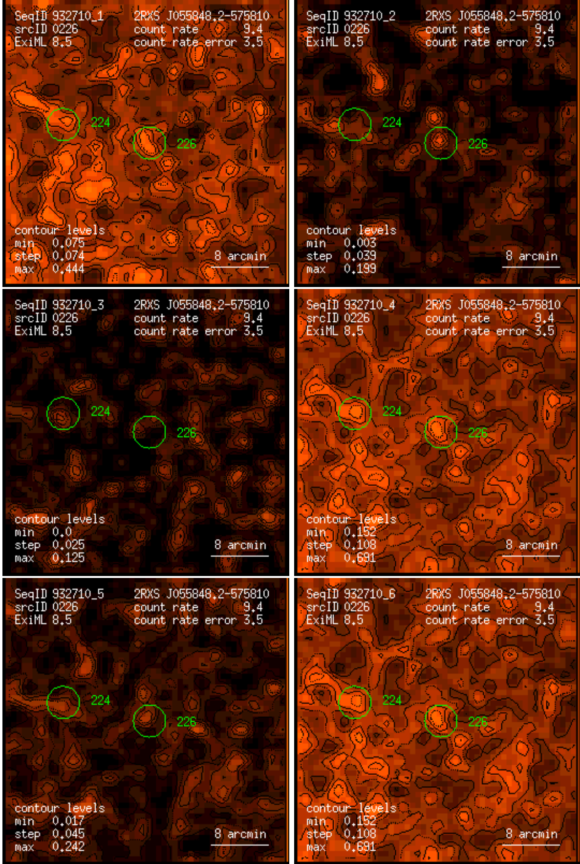
Figure 226: RASS 932710: detection 0226: band rate images, Gaussian filter: (1) PSPC channels 11 – 41, (2) 52 – 90, (3) 91 – 201, (4) 11 – 235, (5) 52 – 201, (6) 11 – 201. Broad band rates in counts/ks. Band rate contour levels in counts/ks/arcmin 2 .
