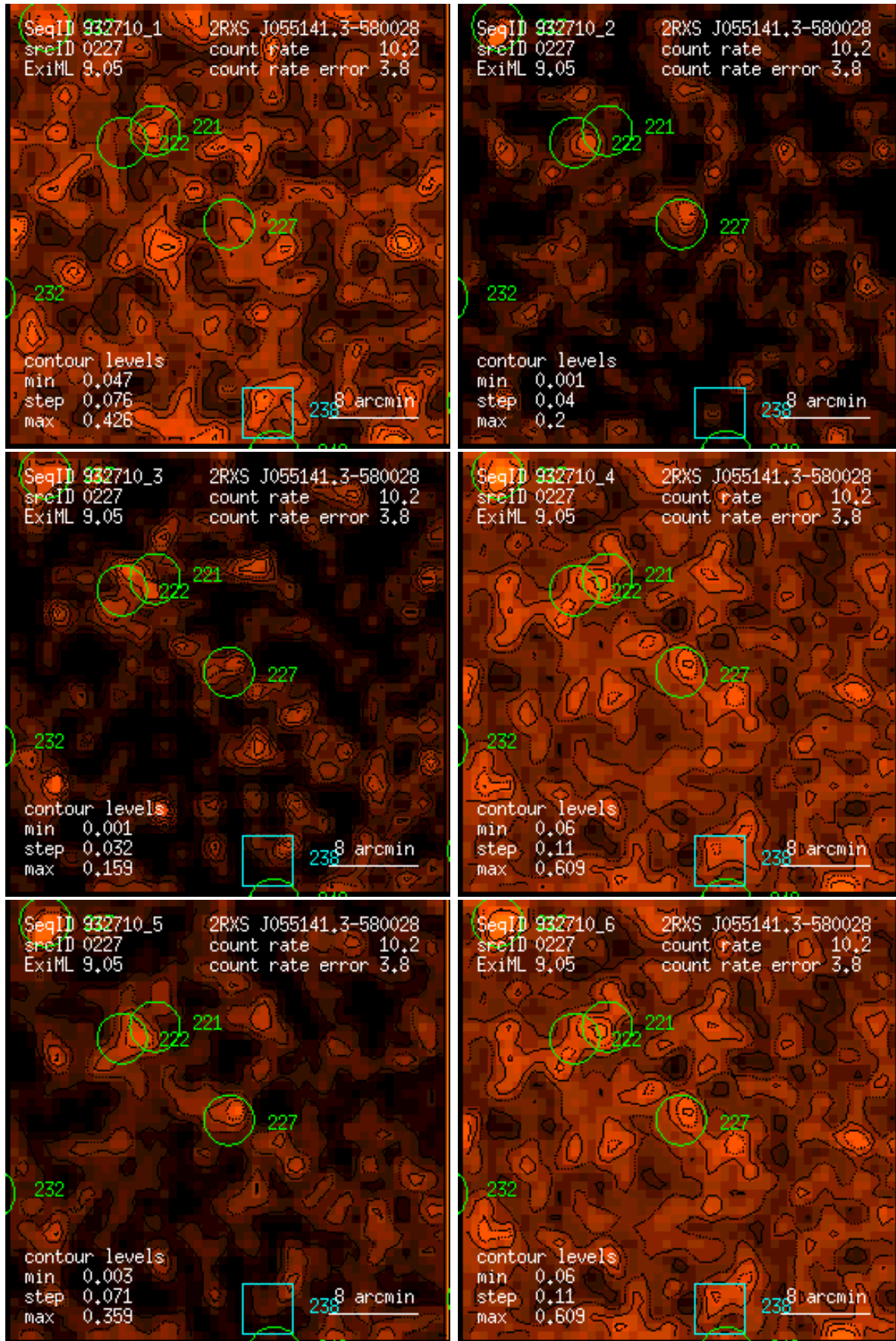
Figure 227: RASS 932710: detection 0227: band rate images, Gaussian filter: (1) PSPC channels 11 – 41, (2) 52 – 90, (3) 91 – 201, (4) 11 – 235, (5) 52 – 201, (6) 11 – 201. Broad band rates in counts/ks. Band rate contour levels in counts/ks/arcmin 2 .
