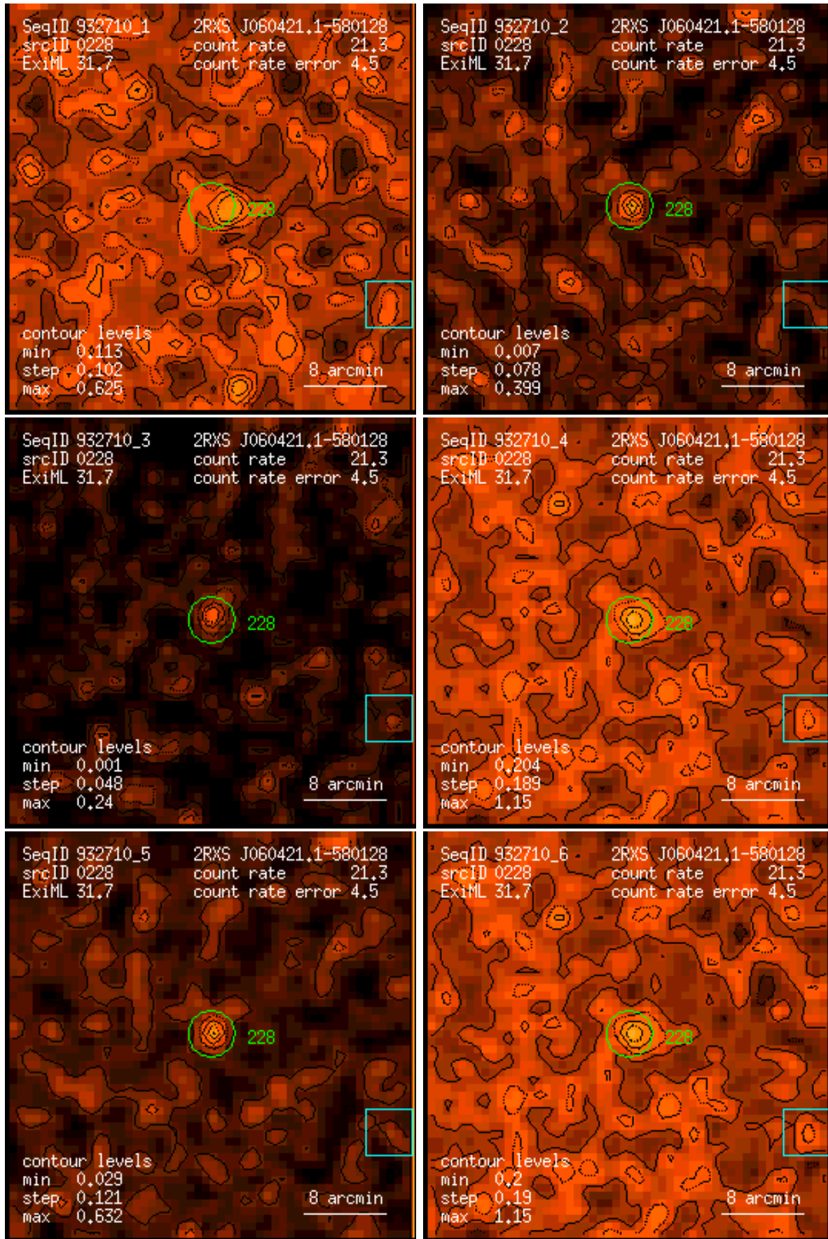
Figure 228: RASS 932710: detection 0228: band rate images, Gaussian filter: (1) PSPC channels 11 – 41, (2) 52 – 90, (3) 91 – 201, (4) 11 – 235, (5) 52 – 201, (6) 11 – 201. Broad band rates in counts/ks. Band rate contour levels in counts/ks/arcmin 2 .
