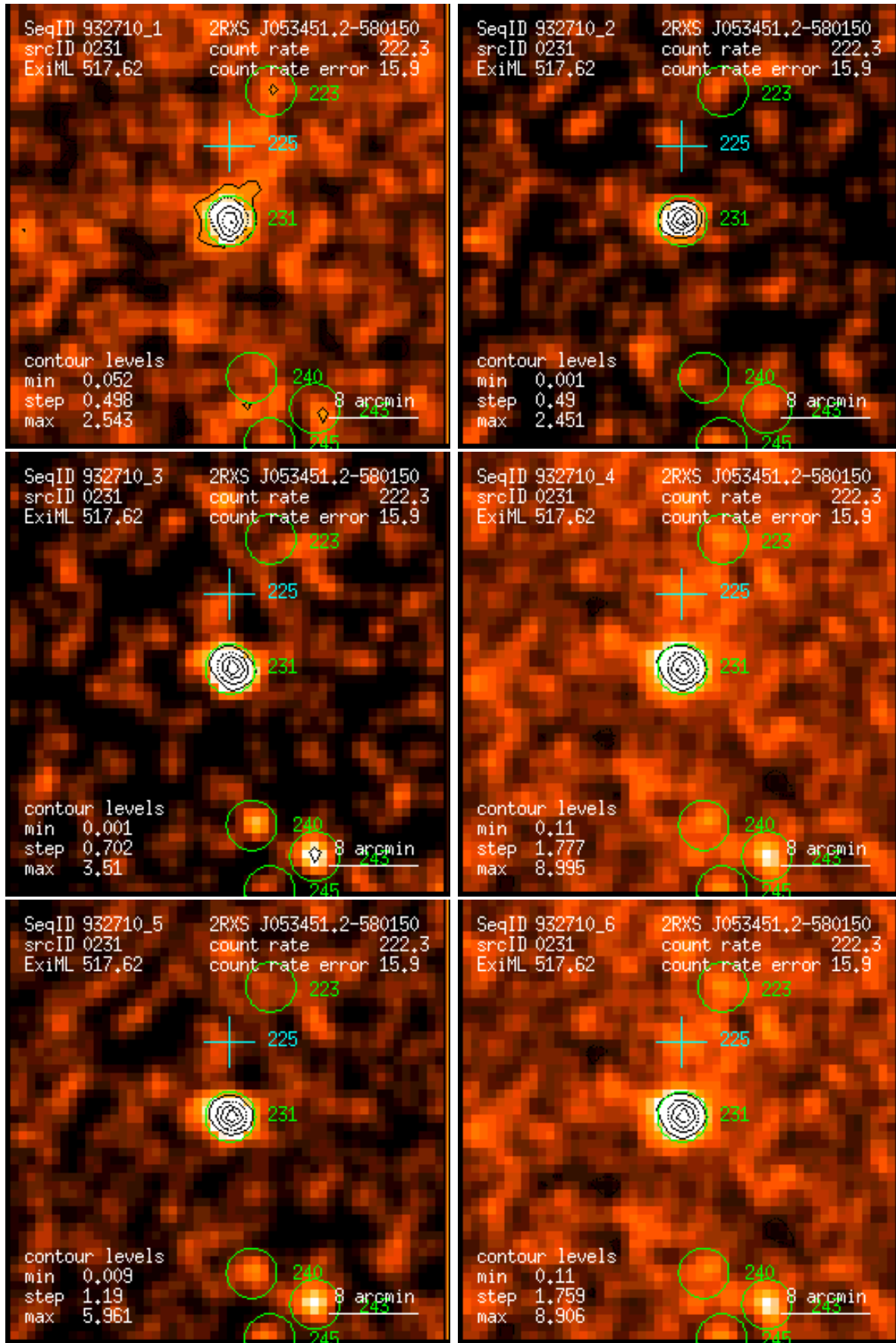
Figure 231: RASS 932710: detection 0231: band rate images, Gaussian filter: (1) PSPC channels 11 – 41, (2) 52 – 90, (3) 91 – 201, (4) 11 – 235, (5) 52 – 201, (6) 11 – 201. Broad band rates in counts/ks. Band rate contour levels in counts/ks/arcmin 2 .
