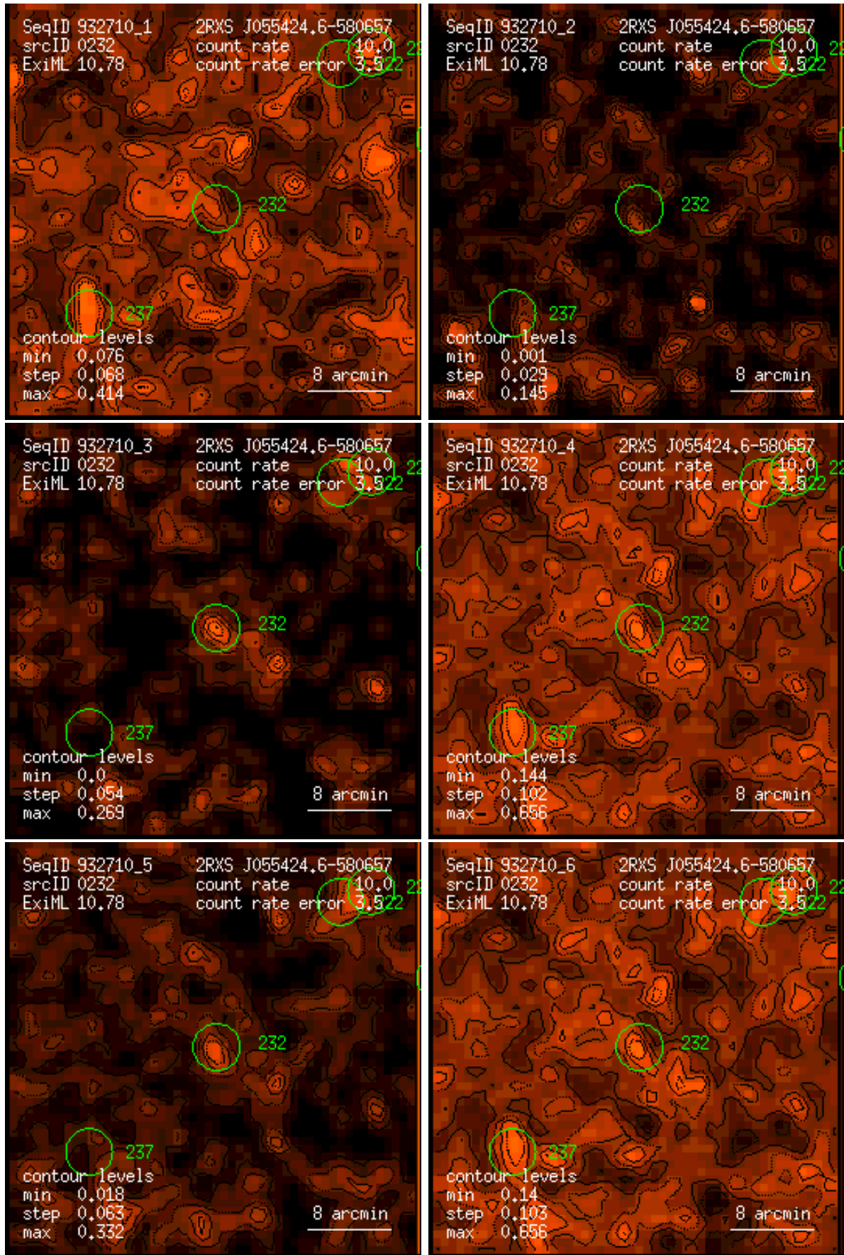
Figure 232: RASS 932710: detection 0232: band rate images, Gaussian filter: (1) PSPC channels 11 – 41, (2) 52 – 90, (3) 91 – 201, (4) 11 – 235, (5) 52 – 201, (6) 11 – 201. Broad band rates in counts/ks. Band rate contour levels in counts/ks/arcmin 2 .
