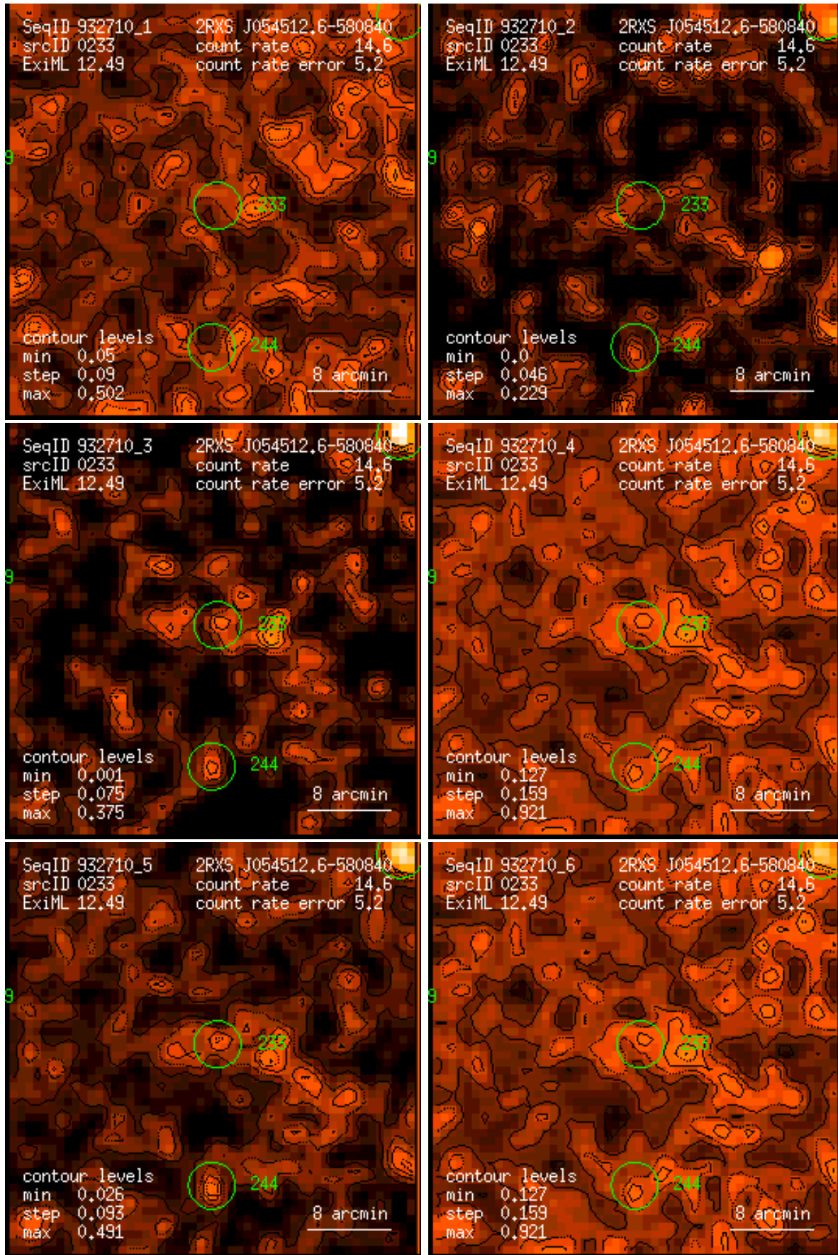
Figure 233: RASS 932710: detection 0233: band rate images, Gaussian filter: (1) PSPC channels 11 – 41, (2) 52 – 90, (3) 91 – 201, (4) 11 – 235, (5) 52 – 201, (6) 11 – 201. Broad band rates in counts/ks. Band rate contour levels in counts/ks/arcmin 2 .
