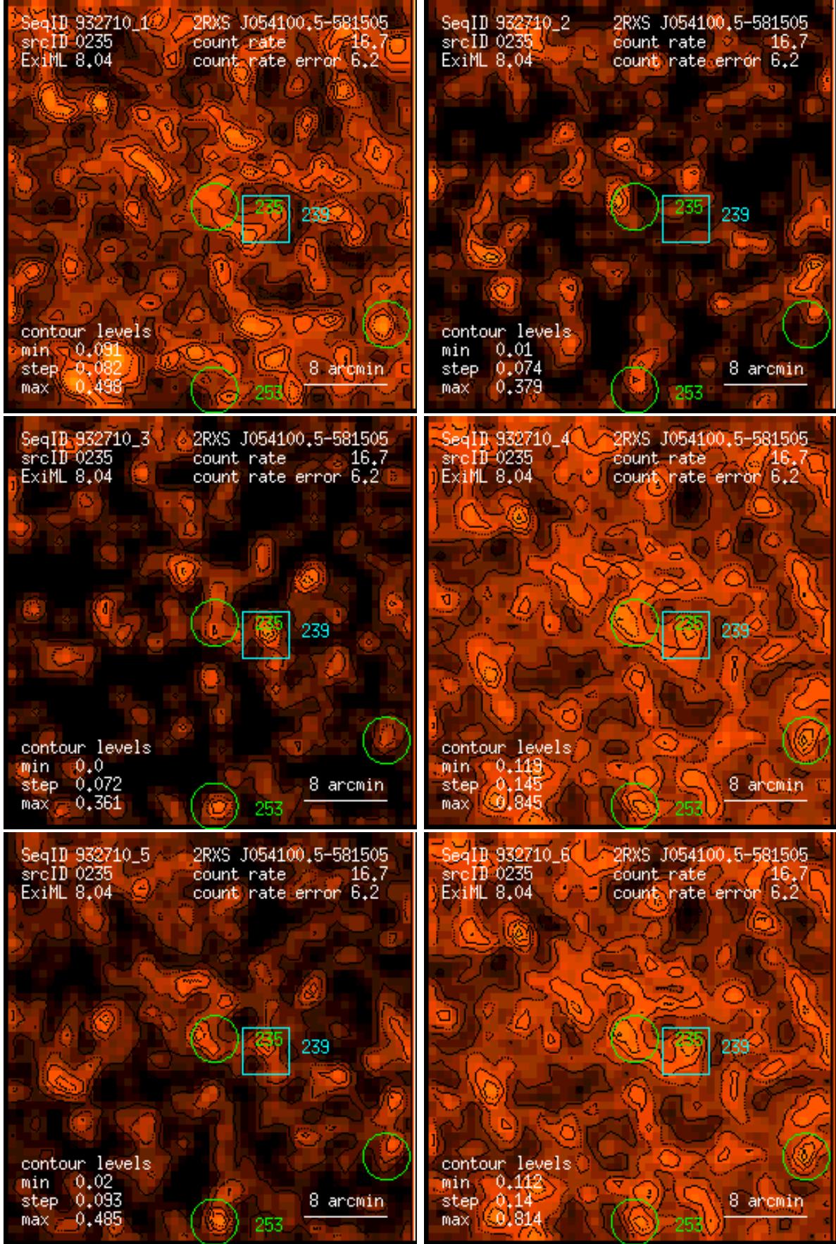
Figure 235: RASS 932710: detection 0235: band rate images, Gaussian filter: (1) PSPC channels 11 – 41, (2) 52 – 90, (3) 91 – 201, (4) 11 – 235, (5) 52 – 201, (6) 11 – 201. Broad band rates in counts/ks. Band rate contour levels in counts/ks/arcmin 2 .
